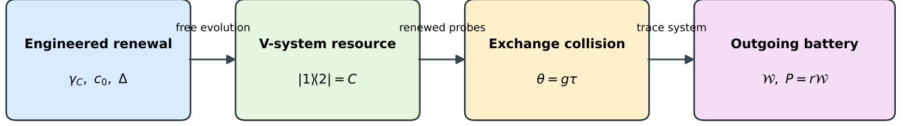
Steady-state coherence is replenished between collisions; extracted work depletes it.
