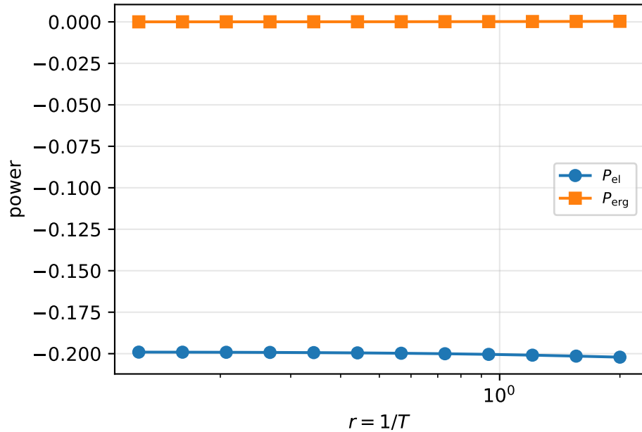
Stage 2: powers vs collision rate ( \theta \approx 0.4 )
