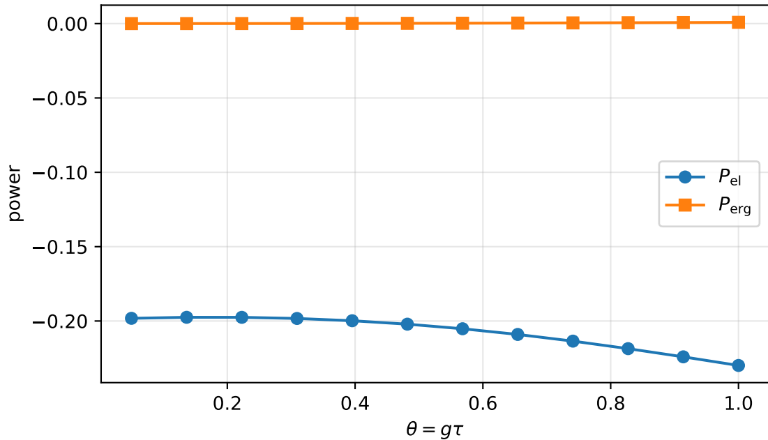
Stage 2: powers vs exchange angle ( T = 1.5 )
