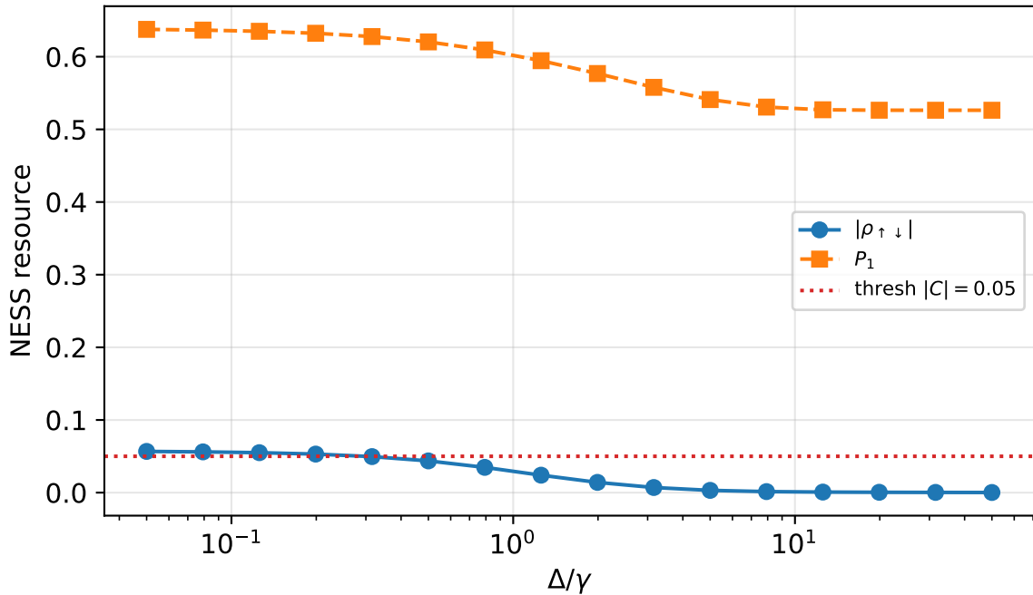
Gate 1: resource vs \Delta/\gamma ( \theta_R = \pi/2 )
