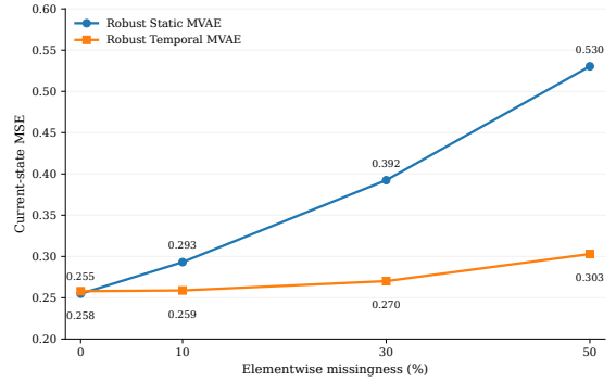
Figure 2: Normalized current-state MSE under elementwise missing-completely-at-random observations. Temporal context provides progressively larger reductions in reconstruction error as the missingness rate increases.
