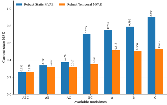
Figure 3: Current-state MSE for all non-empty modality subsets. The Temporal model is approximately tied with the Static model for complete ABC observations but becomes increasingly advantageous as entire modalities are removed.
