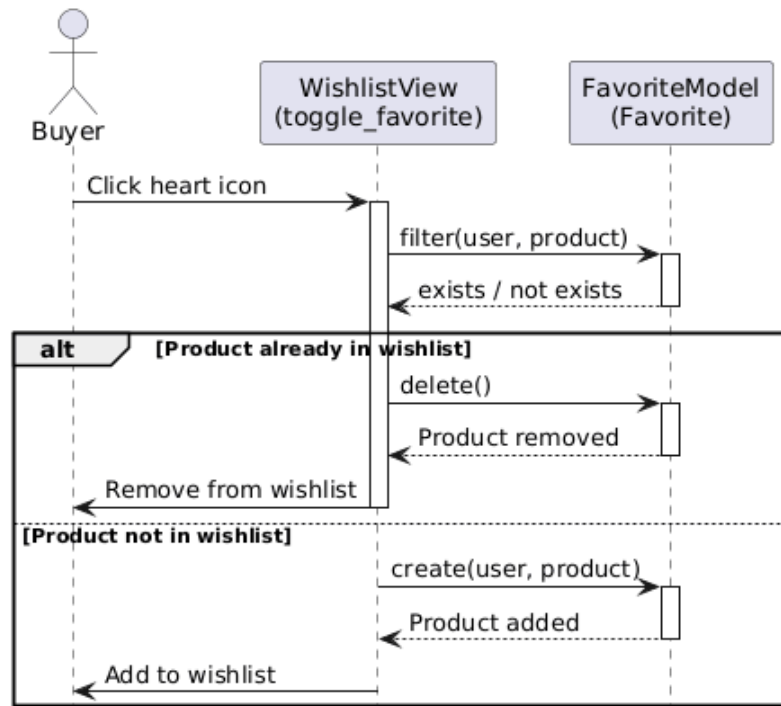
UC-27 Add Product to Wishlist - Sequence Diagram
