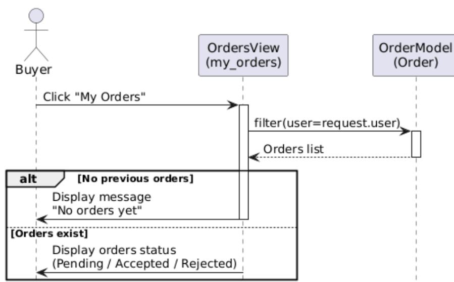
UC-16 View Order Status - Sequence Diagram
