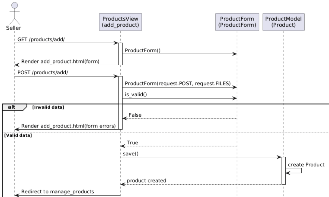
UC-04 Add Product - Sequence Diagram
