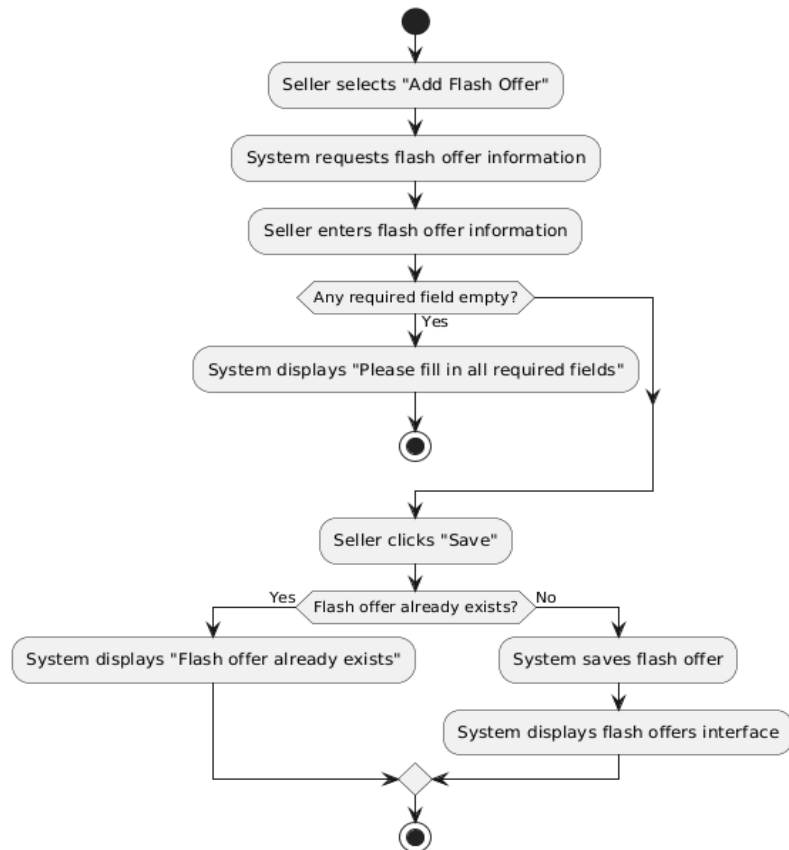
Activity Diagram - Add Flash Offer (UC-24)
