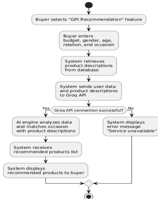
Activity Diagram - Gift Recommendation Using AI (UC-31)
