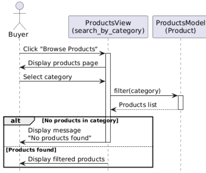
UC-11 Search Products by Category - Sequence Diagram
