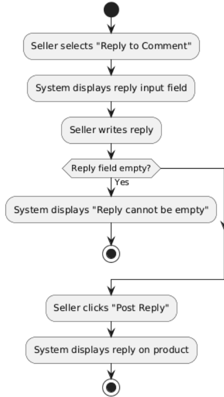
Activity Diagram - Reply to Comment (UC-14)
