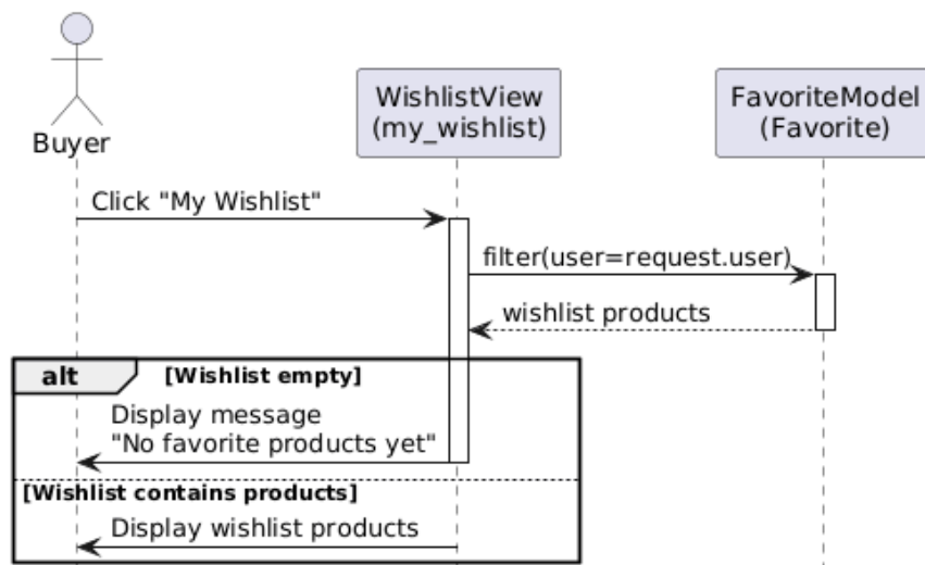
UC-28 View Wishlist - Sequence Diagram
