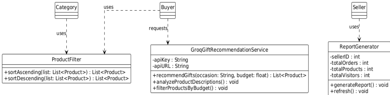
الشكل 78 Services class
