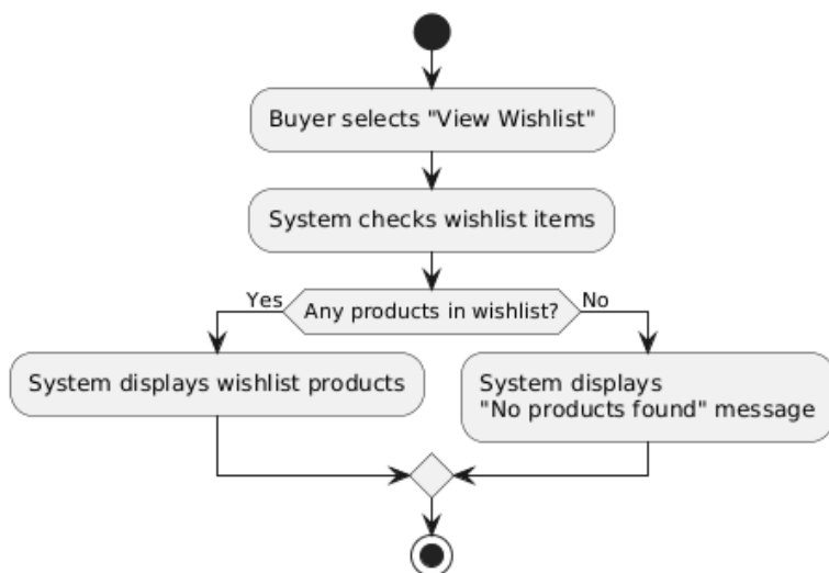
Activity Diagram - View Wishlist (UC-28)
