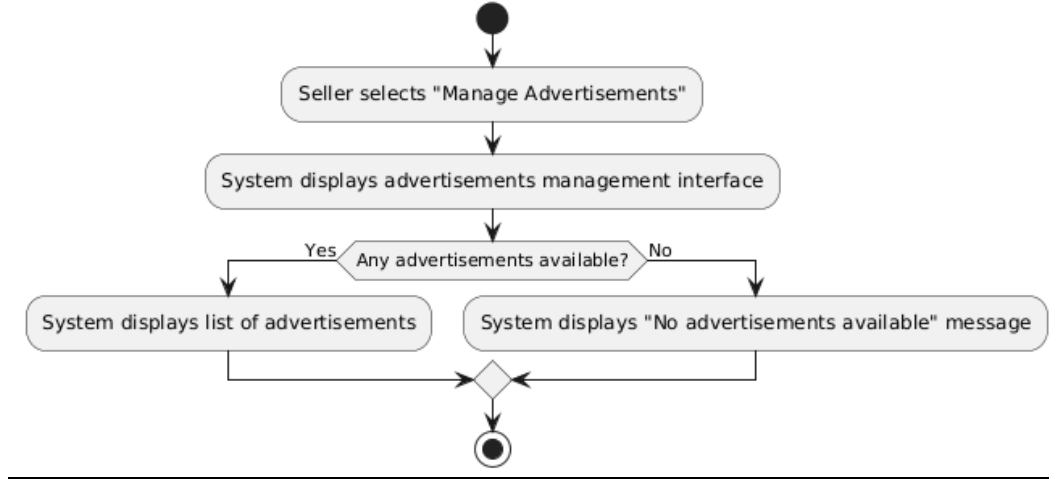
Activity Diagram - Manage Advertisements (UC-19)
