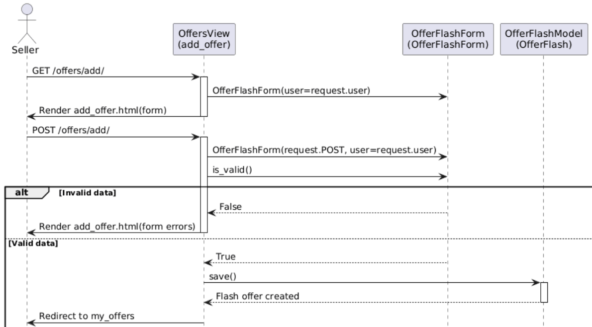
UC-24 Add Flash Offer - Sequence Diagram
