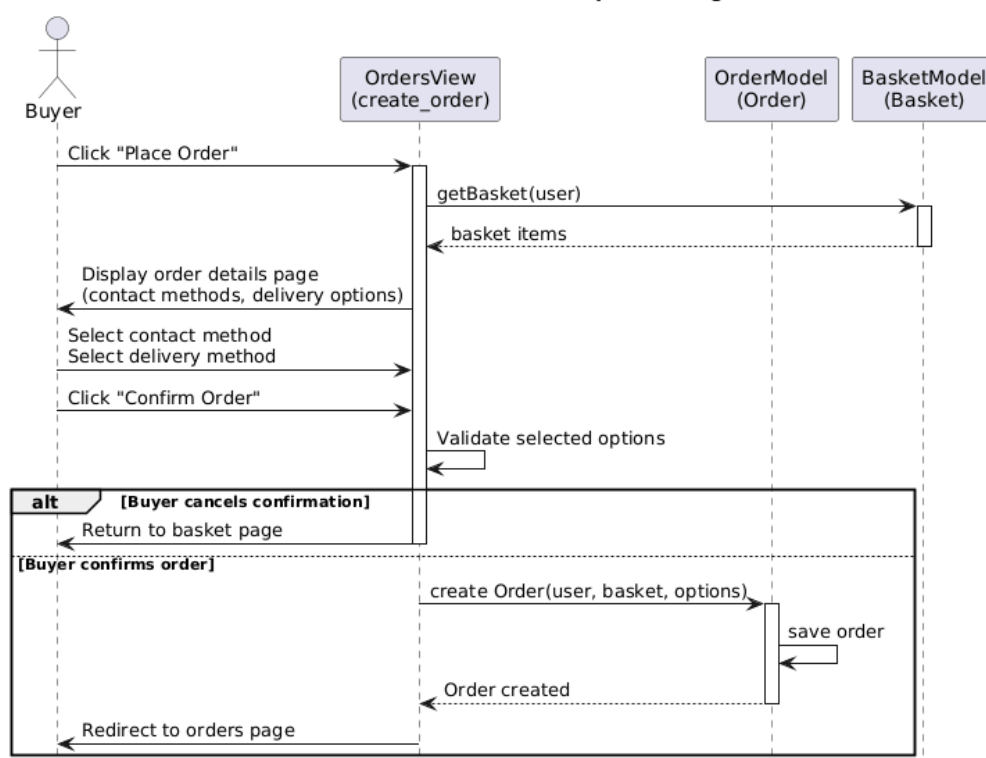
UC-15 Place Purchase Order - Sequence Diagram
