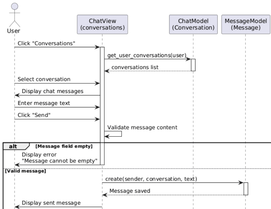
UC-30 Direct Messaging - Sequence Diagram
