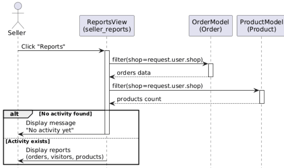
UC-29 View Seller Reports - Sequence Diagram
