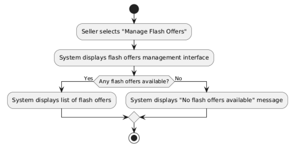
Activity Diagram - Manage Flash Offers (UC-23)
