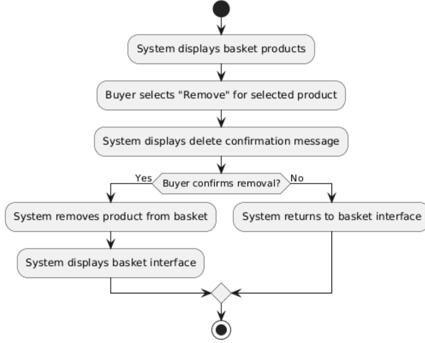
Activity Diagram - Remove Products from Basket (UC-08)
