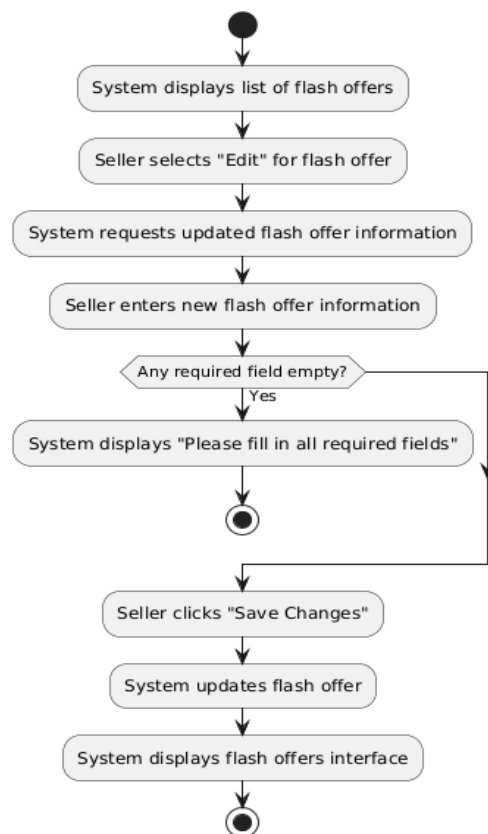
Activity Diagram - Edit Flash Offer (UC-25)
