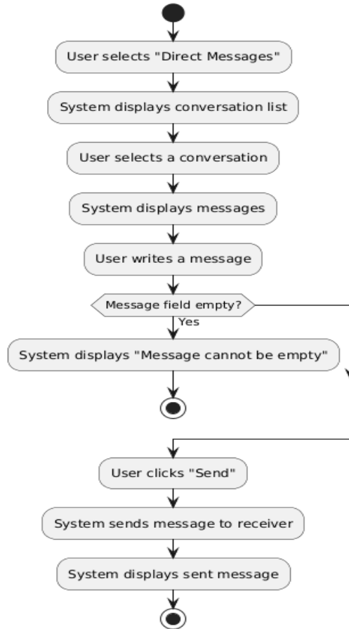
Activity Diagram - Direct Messaging (UC-30)
