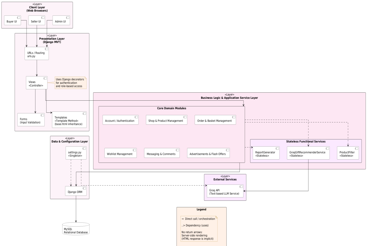
System Architecture Diagram Syrian System for Marketing and Handicrafts
