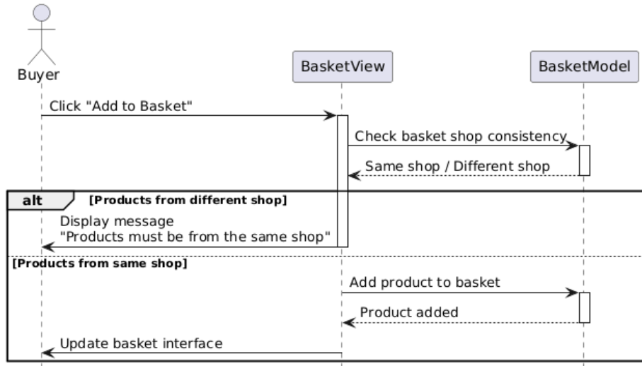
UC-07 Add Products to Basket - Sequence Diagram
