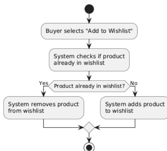
Activity Diagram - Add Products to Wishlist (UC-27)
