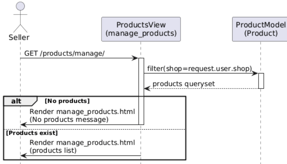
UC-03 Manage Products - Sequence Diagram
