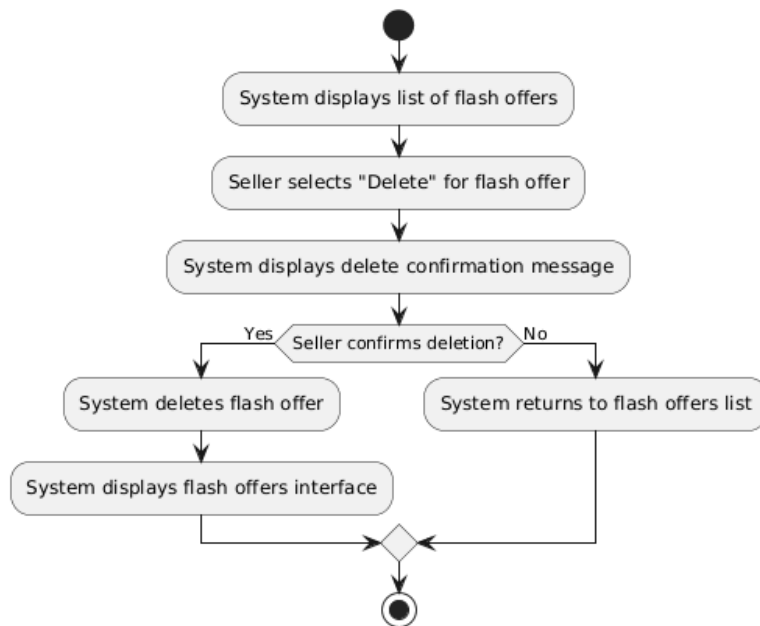
Activity Diagram - Delete Flash Offer (UC-26)
