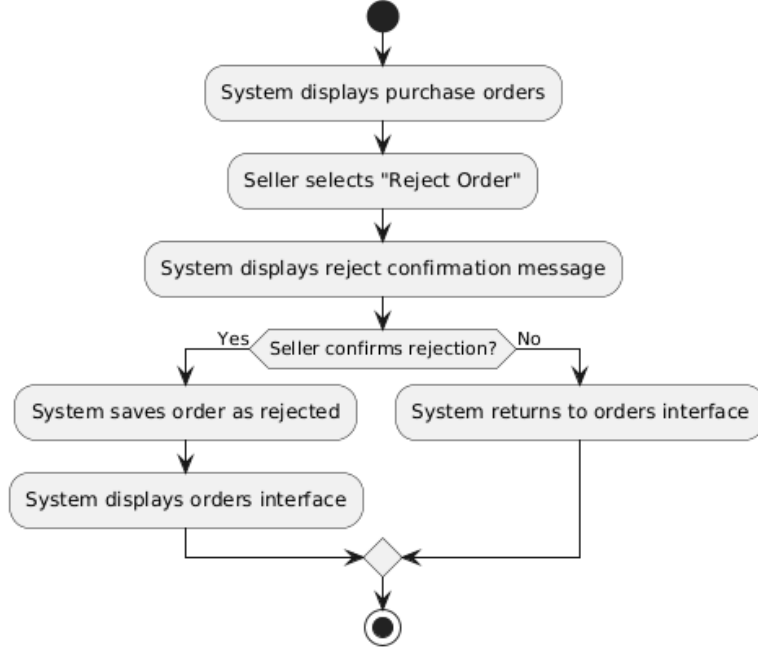
Activity Diagram - Reject Purchase Order (UC-10)
