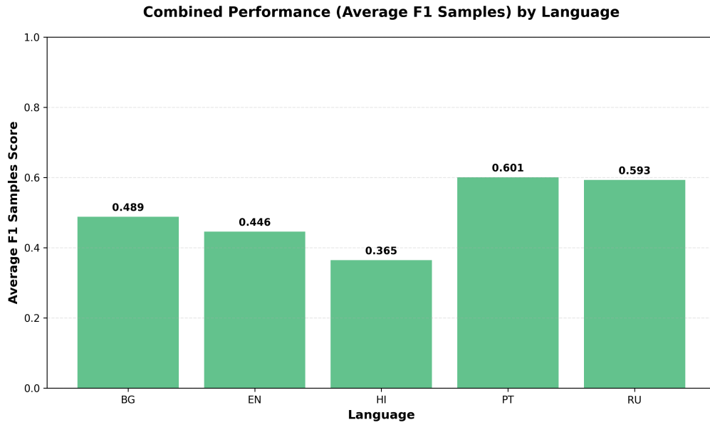
Figure A.8: Combined performance across all languages for the narrative-validation configuration.
