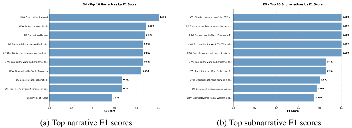
Figure A.4: English performance breakdown for no-validation configuration.
