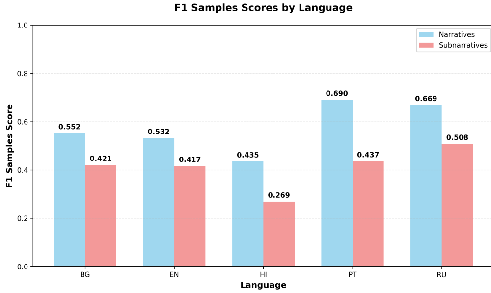
Figure A.16: F1 Samples performance by language for the subnarrative-validation configuration.
