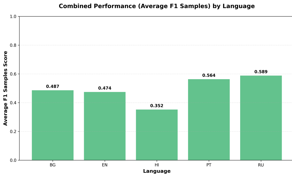
Figure A.15: Combined performance across all languages for the subnarrative-validation configuration.
