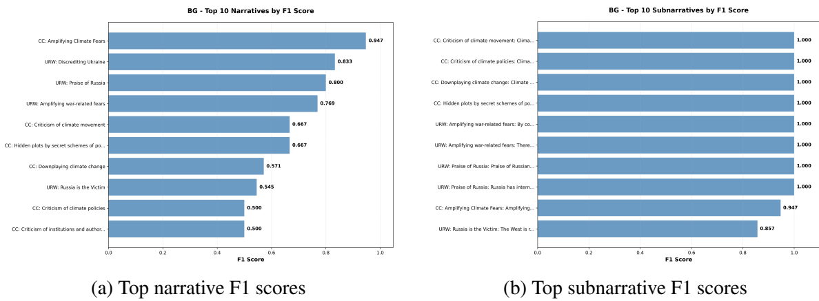
Figure A.17: Bulgarian performance breakdown for subnarrative-validation configuration.
