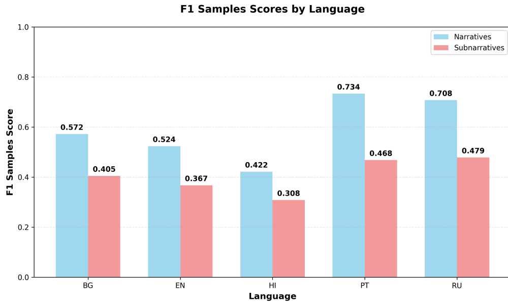
Figure A.9: F1 Samples performance by language for the narrative-validation configuration.
