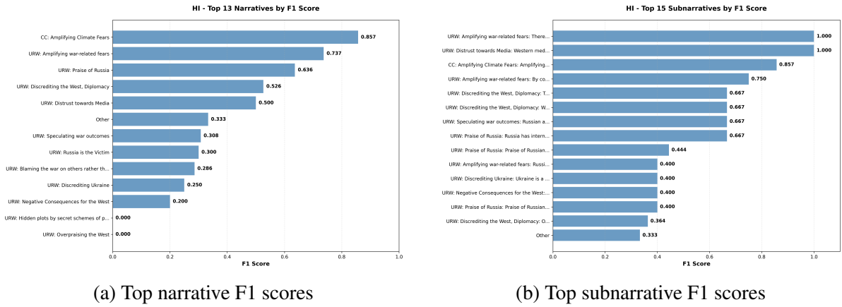
Figure A.12: Hindi performance breakdown for narrative-validation configuration.
