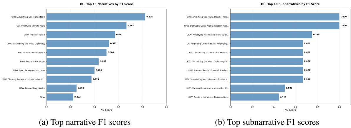
Figure A.19: Hindi performance breakdown for subnarrative-validation configuration.
