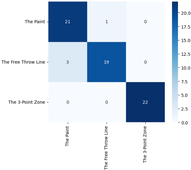
Confusion Matrix (SVC)
