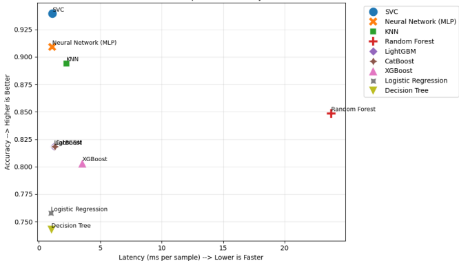
Model Selection: Speed vs. Accuracy
