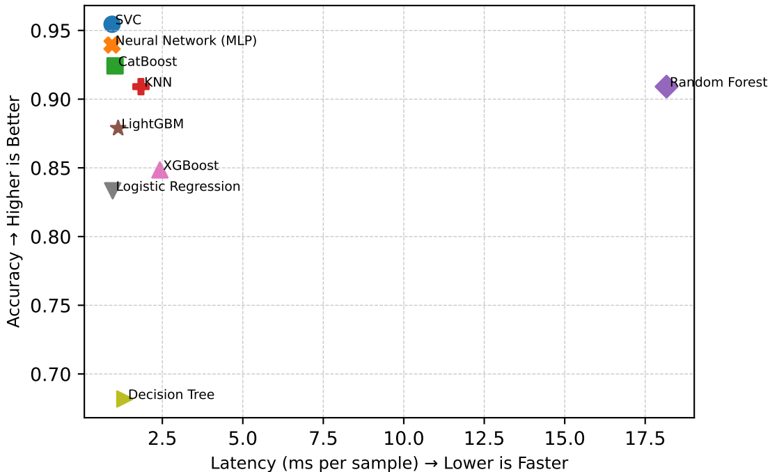
Model Selection: Speed vs. Accuracy
