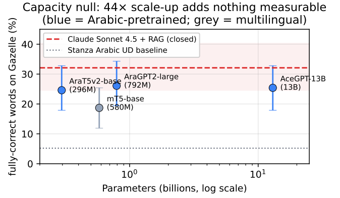
Figure 1: Gazelle fully-correct rate vs. open-weight parameter count (log scale). Three Arabic-pretrained models (296M, 792M, 13B; blue) train to statistically indistinguishable performance — every pairwise McNemar p=1.000 . The closed-system frontier (Sonnet RAG, dashed red) sits 7–8 pp above. Multilingual mT5 (grey) trails by paired-significant margin. Scale within Arabic-pretrained open weights does not move the headline.
