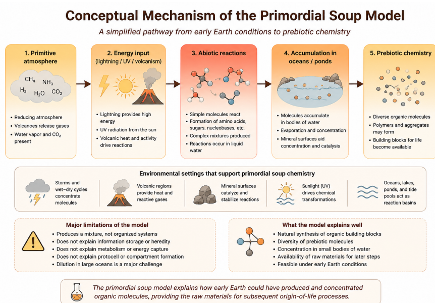
Figure 2.1: Conceptual mechanism of the primordial soup model.
