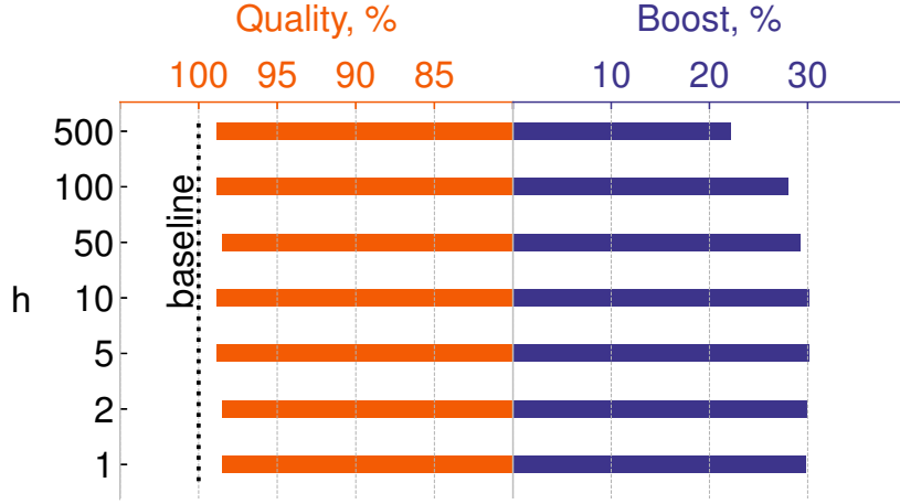
Figure 5: Sensitivity analysis of ID-LoRA to h hyperparameter. \alpha is 0.6, importance metric is cosine similarity.
