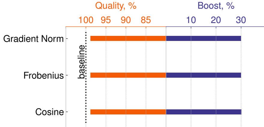
Figure 6: Sensitivity analysis of ID-LoRA to considered importance metrics. \alpha is 0.6, h is 10.
