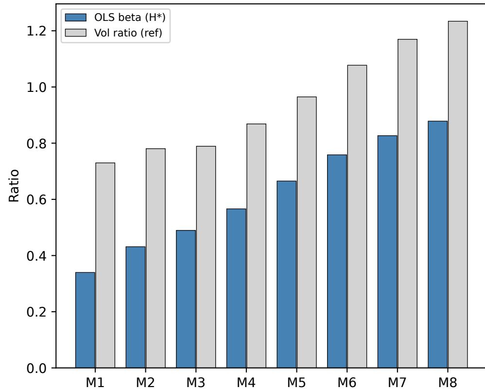
Hedge Ratio H^* vs Vol Ratio
