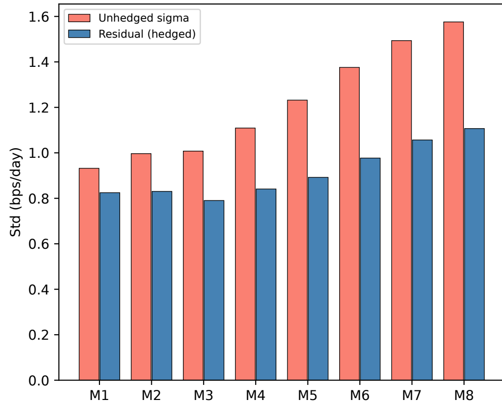
Risk Before vs After Hedge (bps/day)
