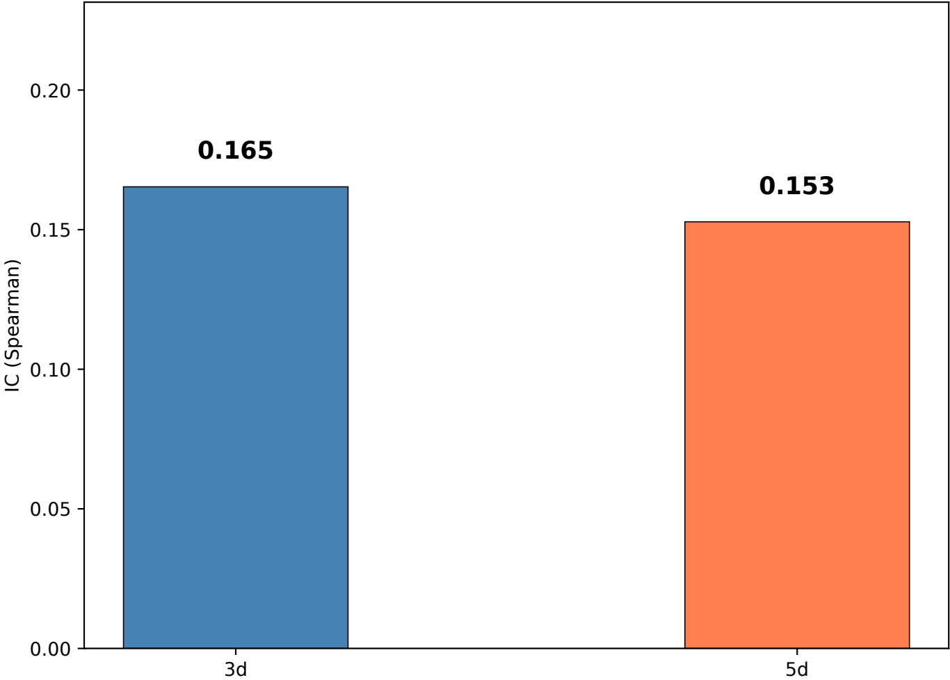
OOS IC by Horizon
