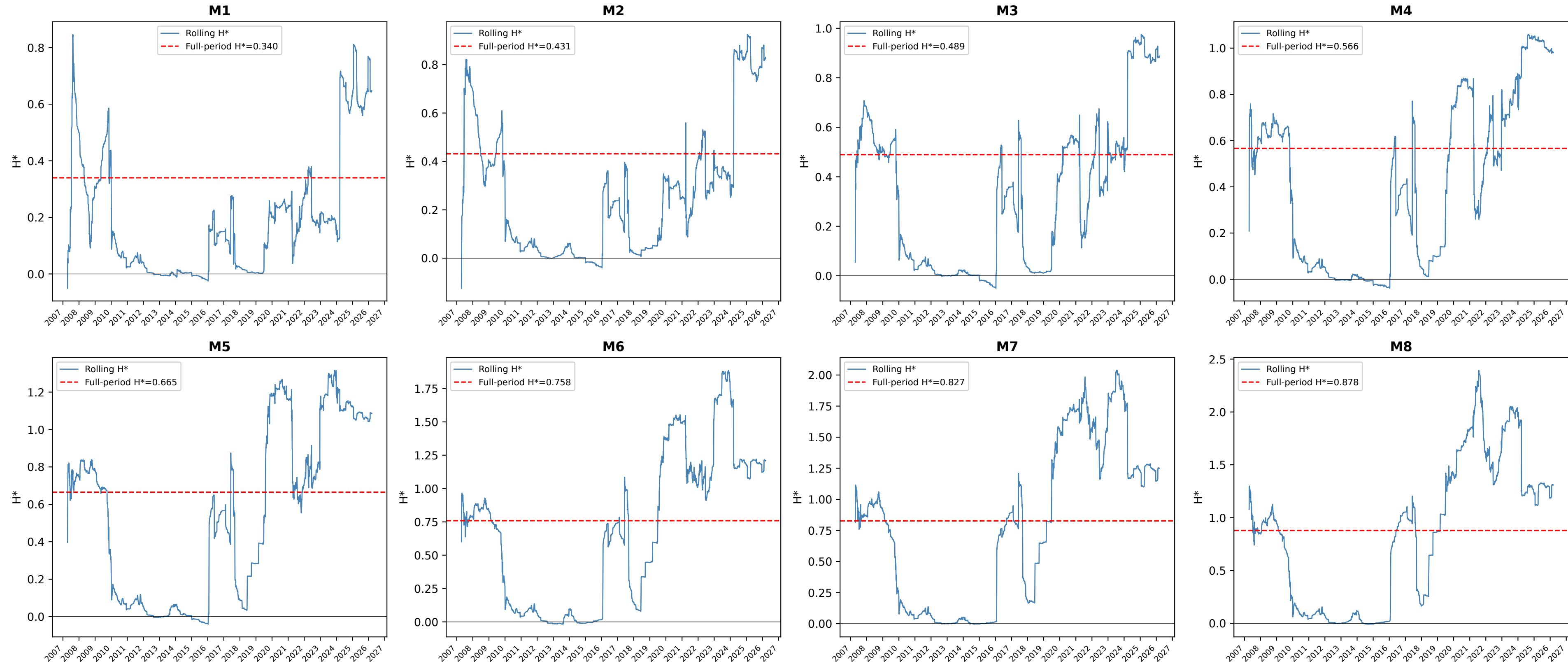
Rolling Hedge Ratio H^* (252-day window) — M_n vs T12
