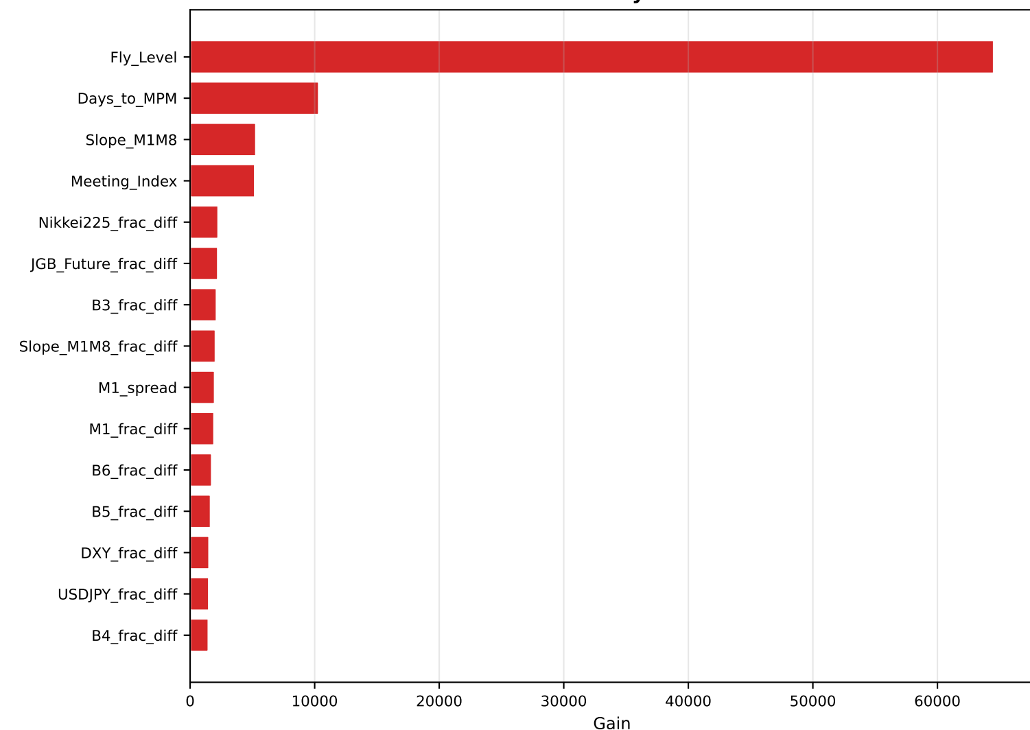
Feature Importance (gain, last fold, top 15) | 2026-03-12
