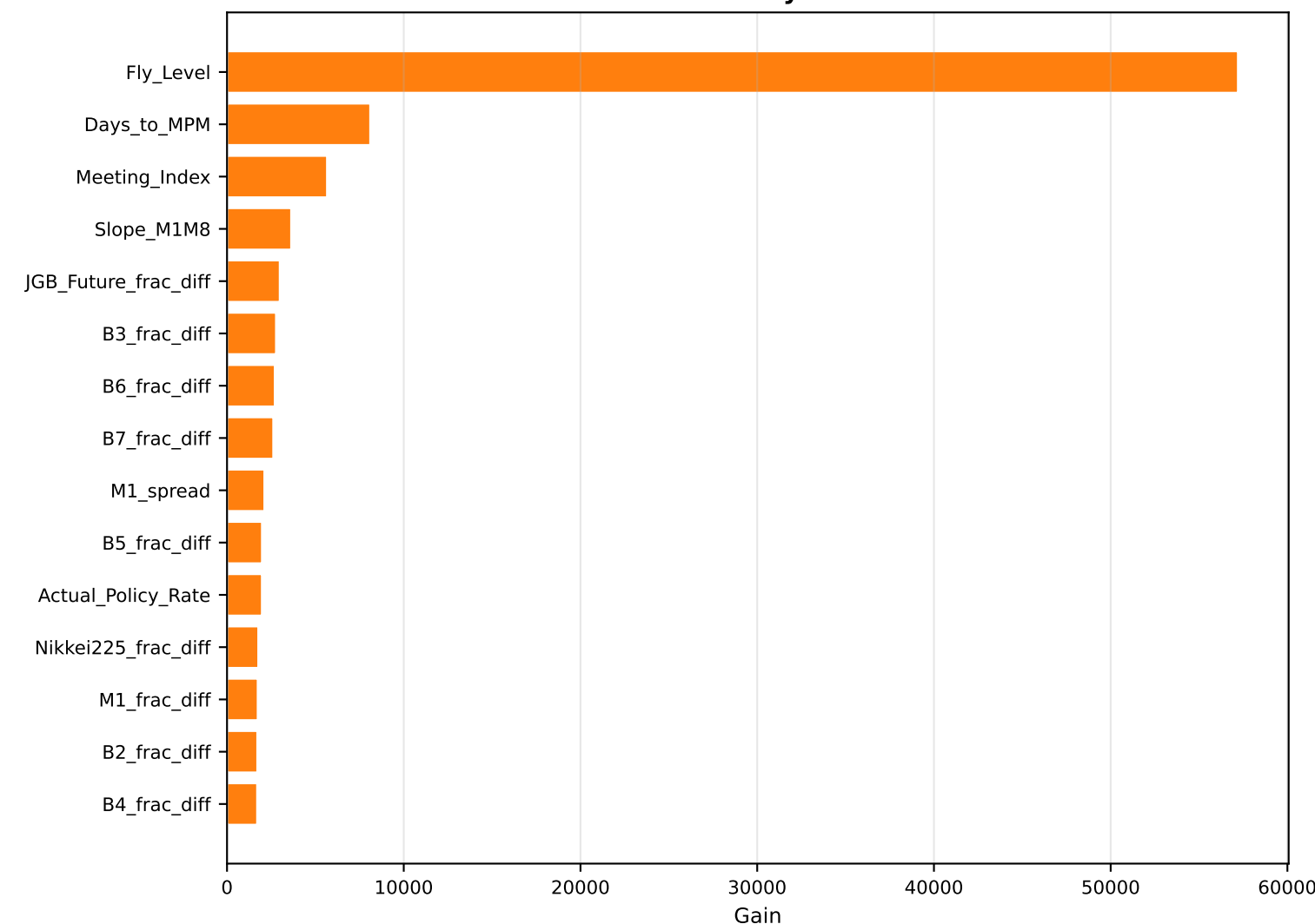
Feature Importance (gain, last fold, top 15) | 2026-03-23
