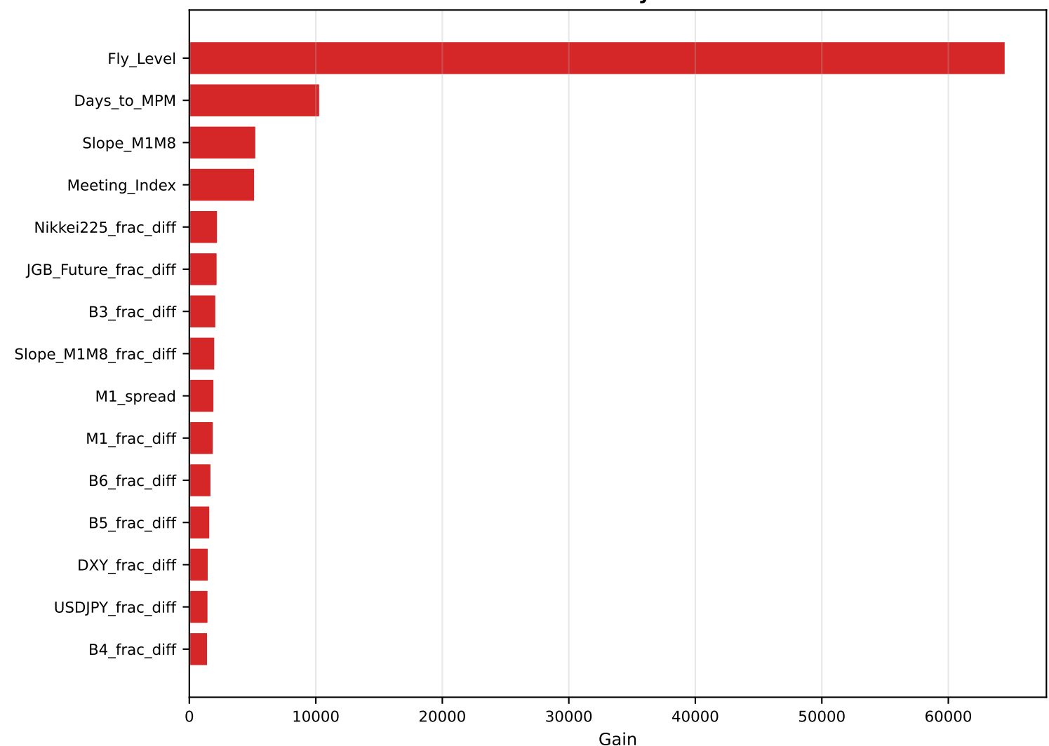
Feature Importance (gain, last fold, top 15) | 2026-03-23
