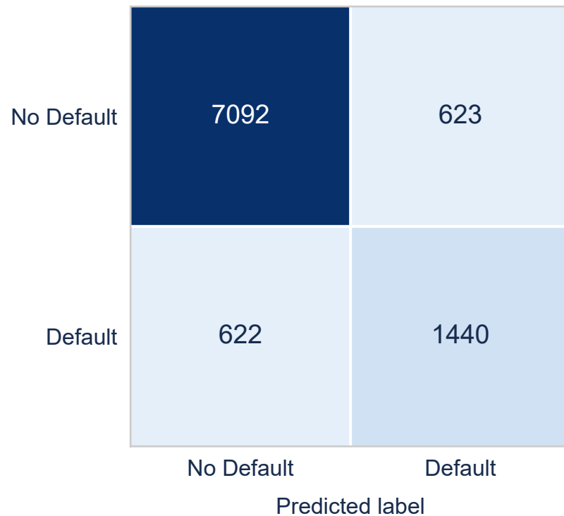
XGBoost
