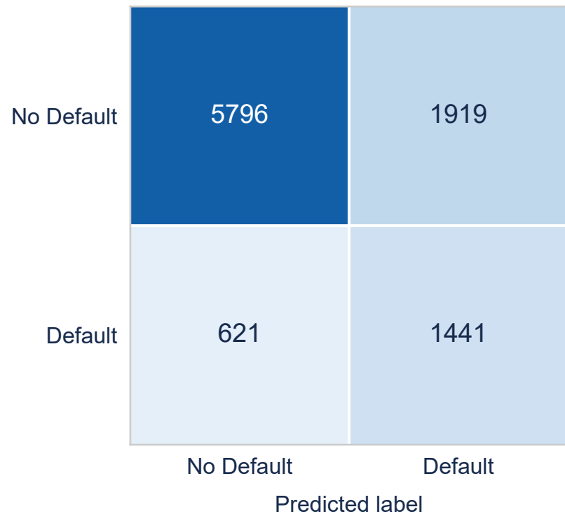
Logistic Regression
