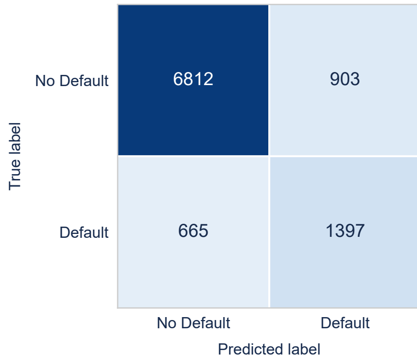
Random Forest
