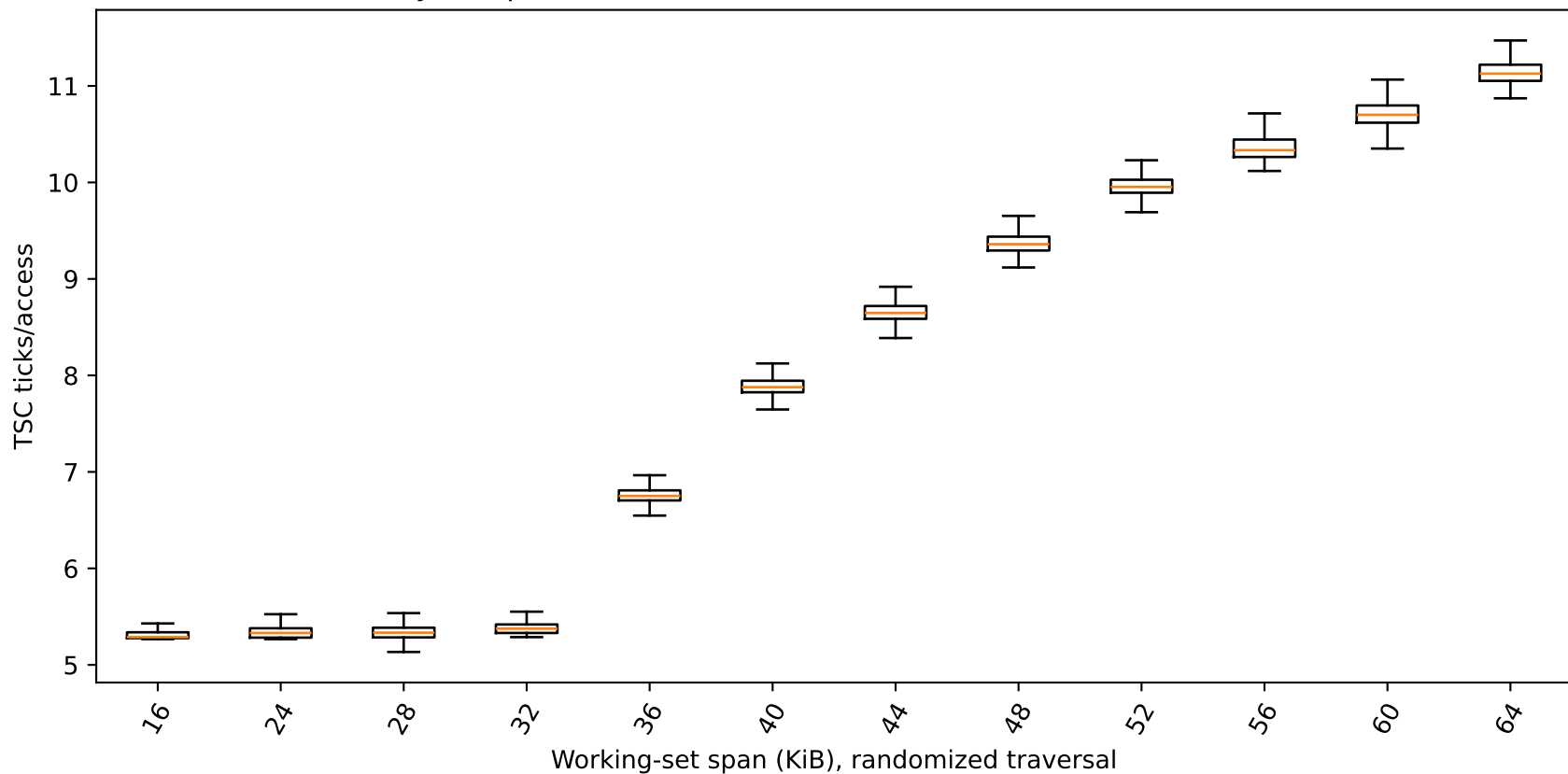
charnwood.ece.ncsu.edu Tukey box plots; outliers retained in raw files and counted in CSV
