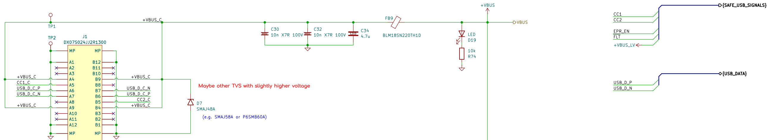
USB-C 3.2 Gen2 48V 5A SMD receptacle
