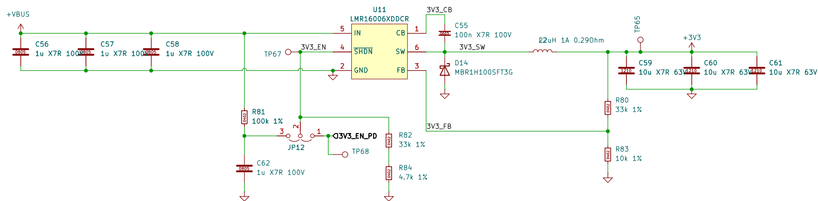
3.3V 600mA 700kHz Buck Regulator
