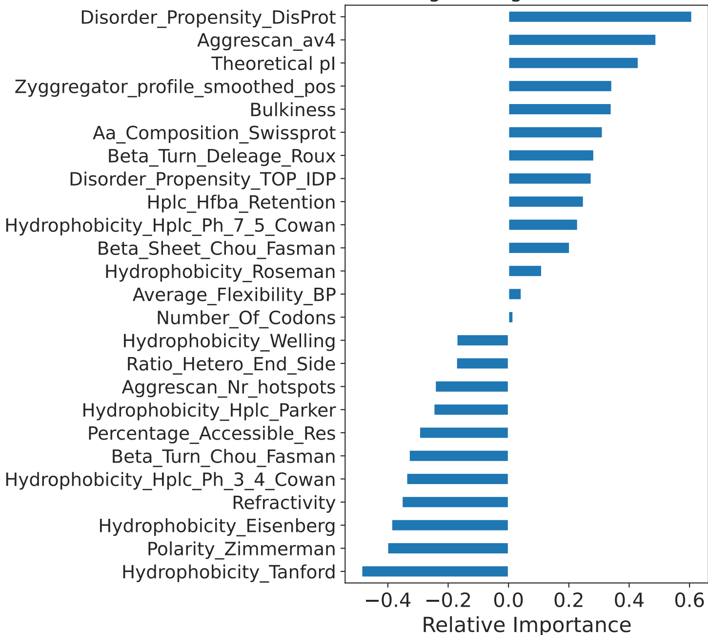
LogisticReg coefficients
