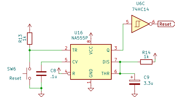
Debounced Reset
