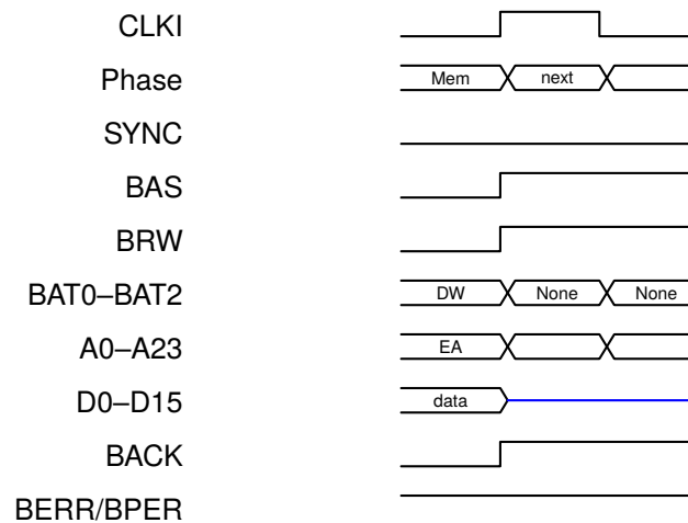
Figure F.4: Data write cycle with no wait state
