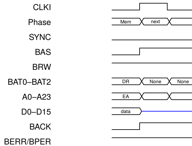
Figure F.3: Data read cycle with no wait state
