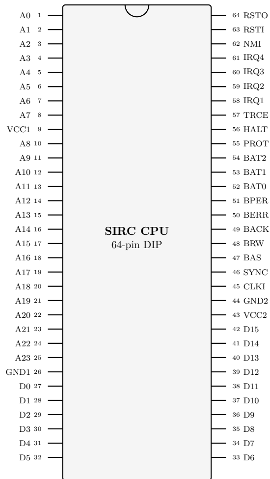
Figure F.1: SIRC CPU 64-pin DIP pinout, top view
