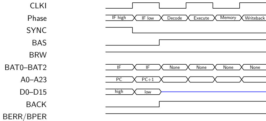
Figure F.8: Complete register-only ALU instruction with no wait states
