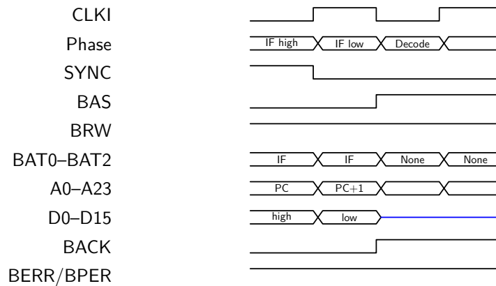
Figure F.2: Instruction-fetch high-word and low-word reads with no wait states
