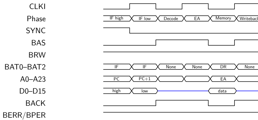
Figure F.9: Complete LOAD instruction with no wait states
