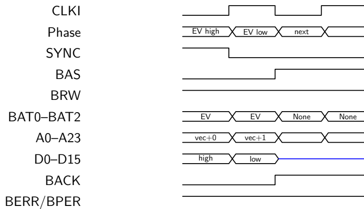
Figure F.5: Exception-vector fetch with high-word then low-word reads
