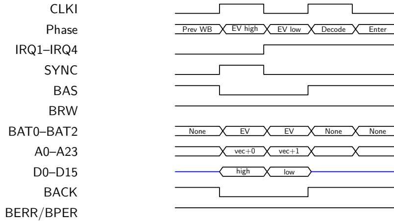
Figure F.11: Enabled IRQ sampled at an instruction boundary and dispatched with no wait states
