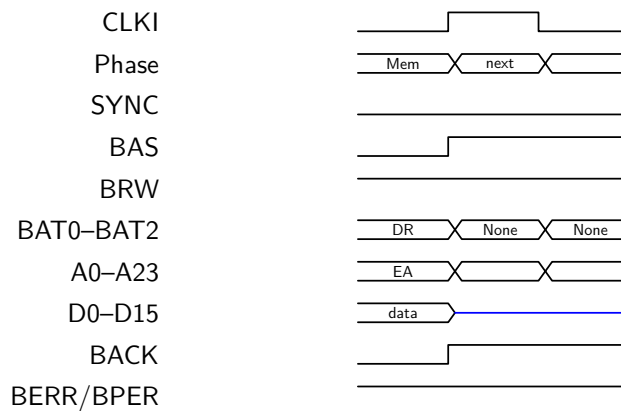
Figure F.3: Data read cycle with no wait state
