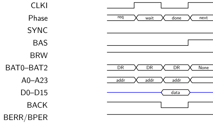
Figure F.6: Wait-state insertion when no bus response is asserted
