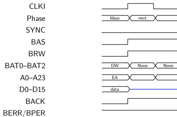
Figure F.4: Data write cycle with no wait state
