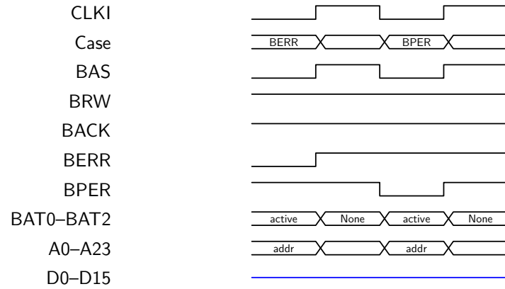
Figure F.7: Bus-error and bus-protection abort timing
