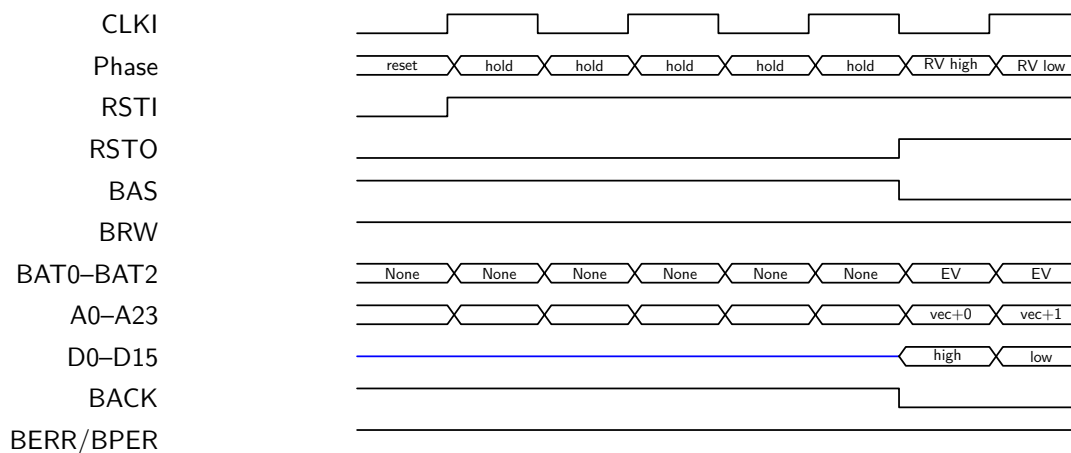
Figure F.10: Hardware reset with one-cycle RSTI assertion and reset-vector fetch
