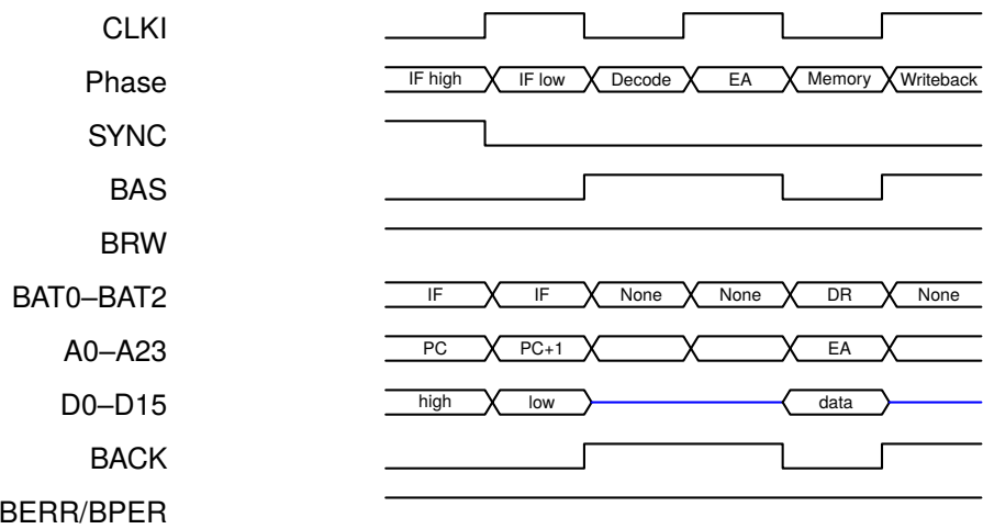
Figure F.9: Complete LOAD instruction with no wait states
