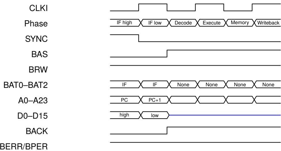
Figure F.8: Complete register-only ALU instruction with no wait states
