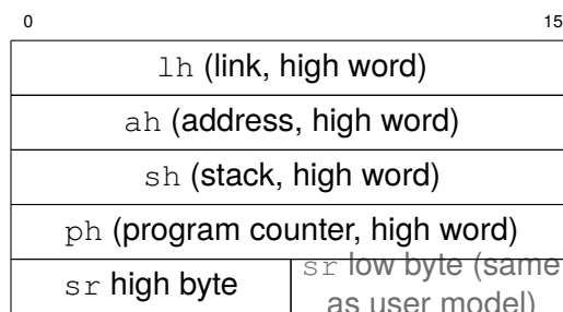
Figure 3.2: Supervisor Programming Model Supplement
