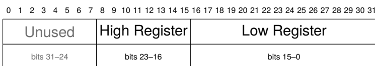
Figure 3.3: Address Register Pair Formation
