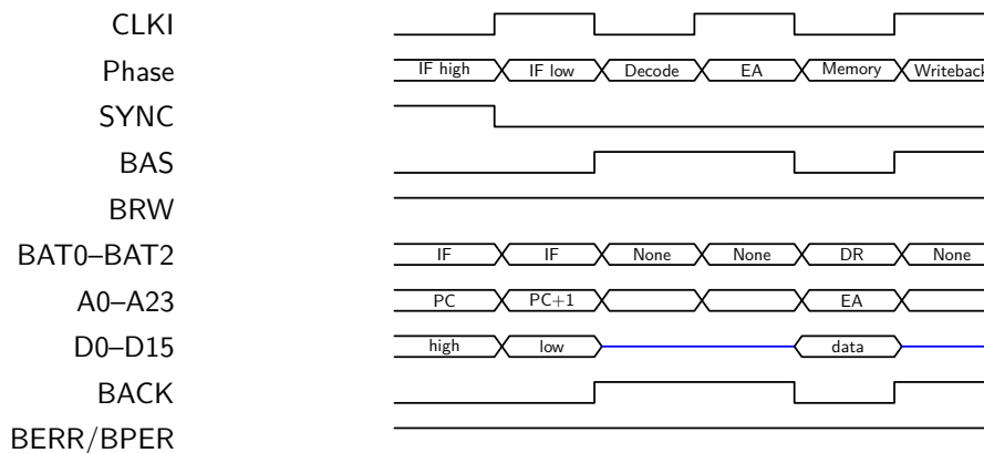
Figure F.9: Complete LOAD instruction with no wait states
