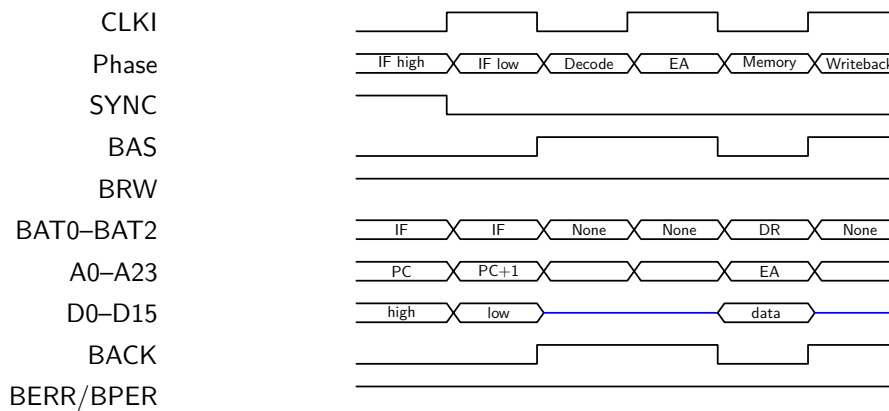
Figure 2.10: Complete LOAD instruction with no wait states
