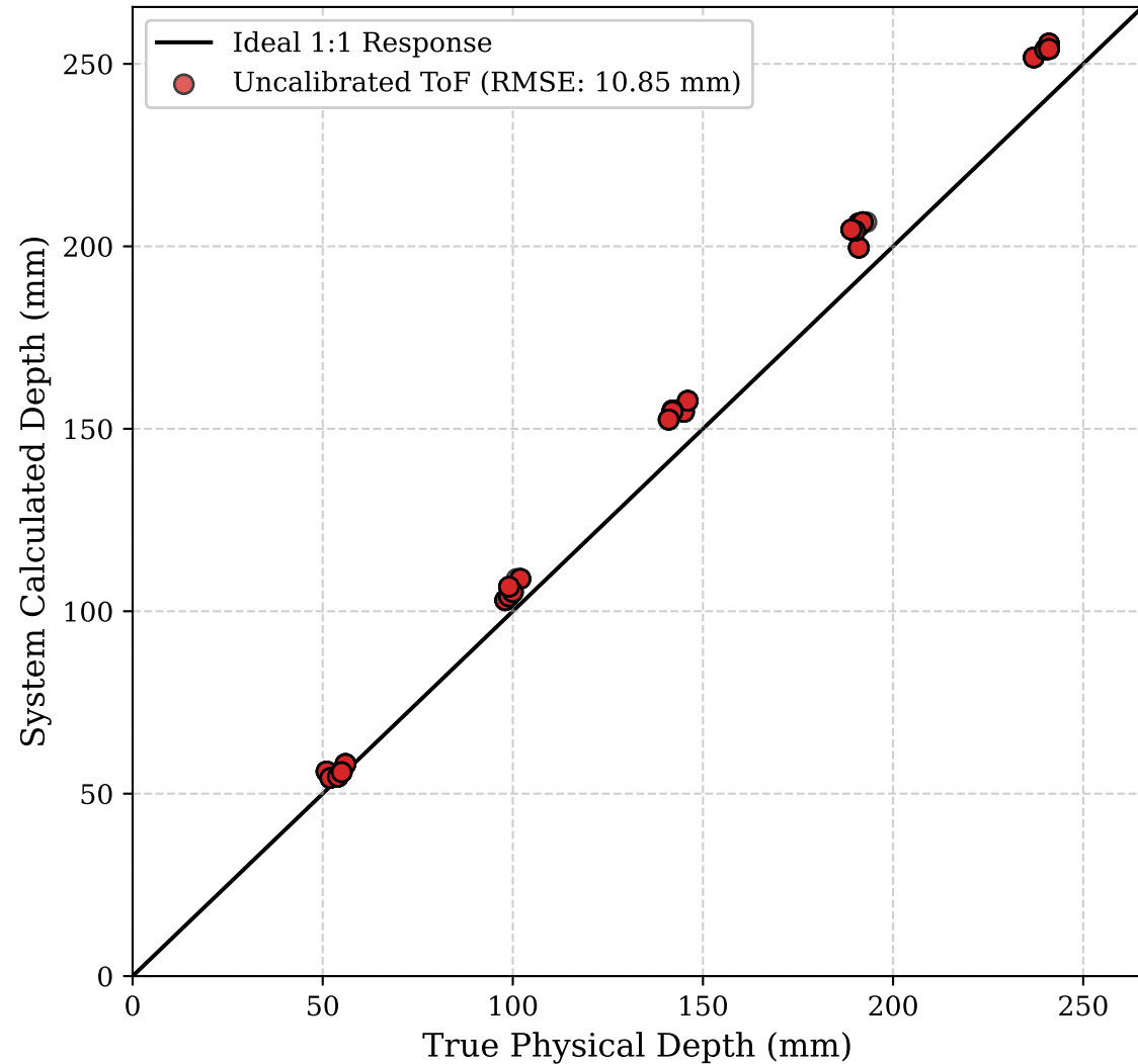
System Measurement Linearity
