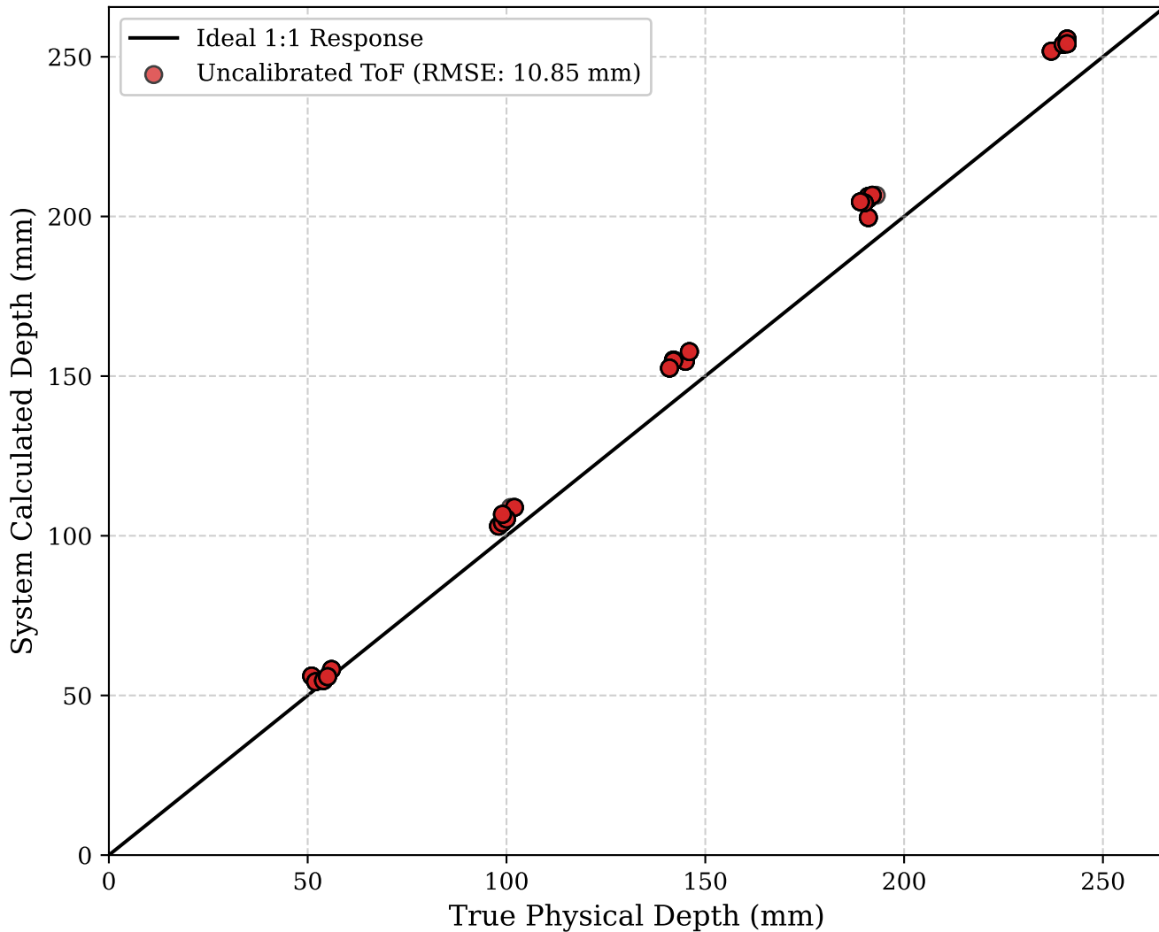
Time-of-Flight Sensor Measurement Linearity
