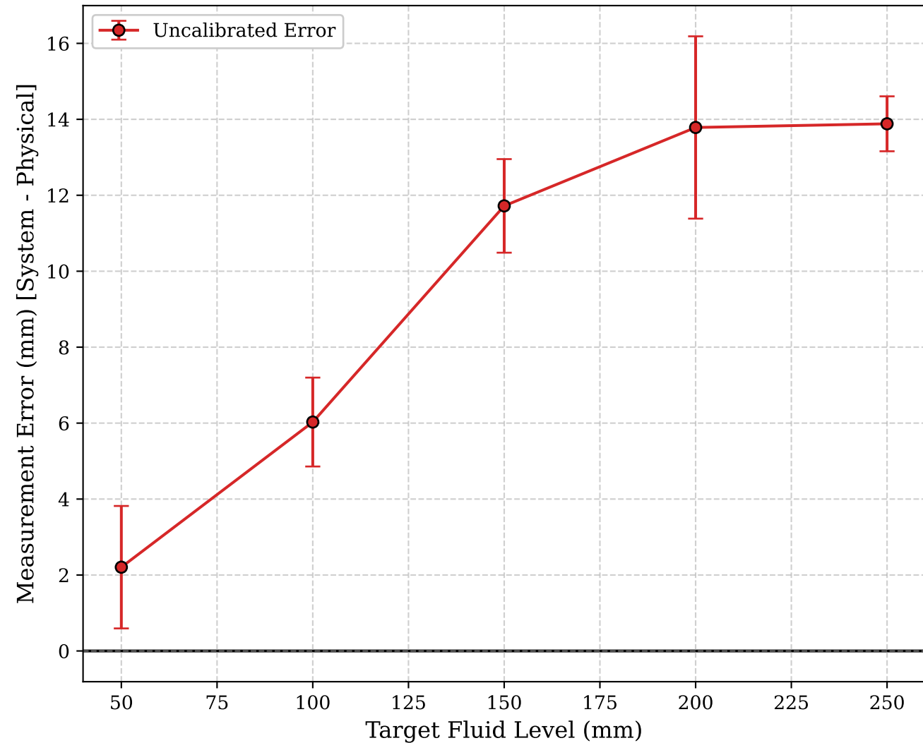
Absolute Measurement Error vs. Fluid Level
