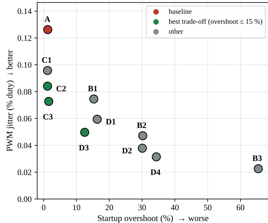
(c) Trade-off, all 11 settings
