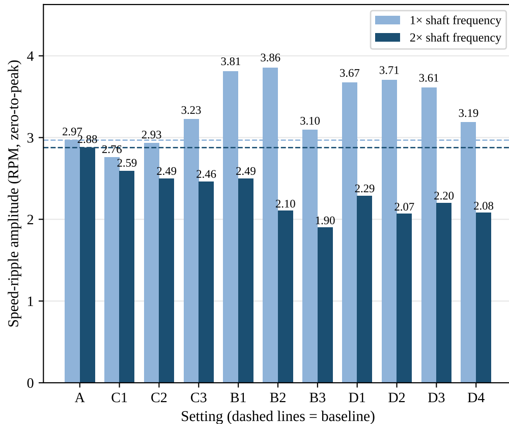
(b) Speed ripple at 1× and 2× shaft frequency
