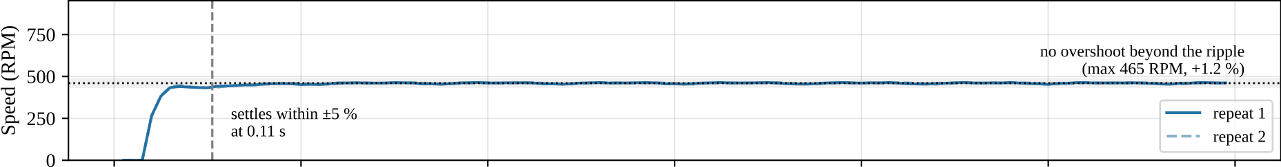
C1: Kp 1.2 → overshoot 1.2 %, settles in 0.11 s
