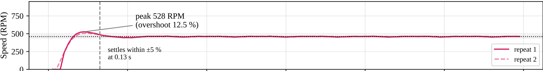
D3: Kp 1.0, α 0.5 → overshoot 12.5 %, settles in 0.13 s
