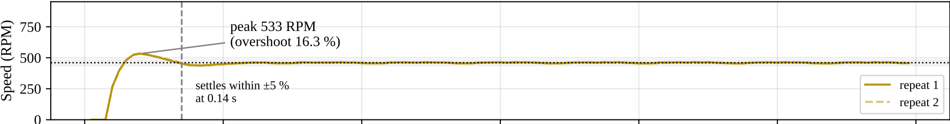
D1: Kp 1.2, α 0.5 → overshoot 16.3 %, settles in 0.14 s
