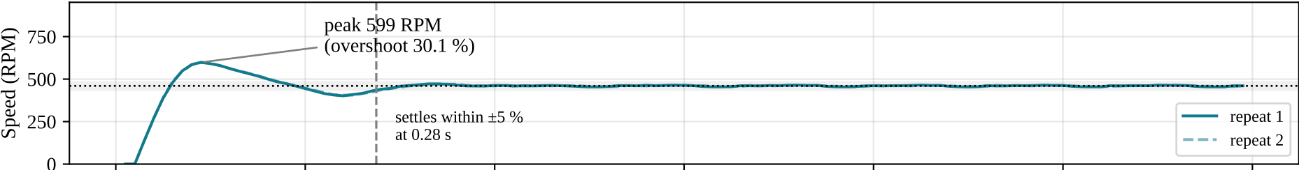
D2: Kp 1.2, α 0.3 → overshoot 30.1 %, settles in 0.28 s
