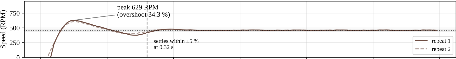
D4: Kp 1.0, α 0.3 → overshoot 34.3 %, settles in 0.32 s
