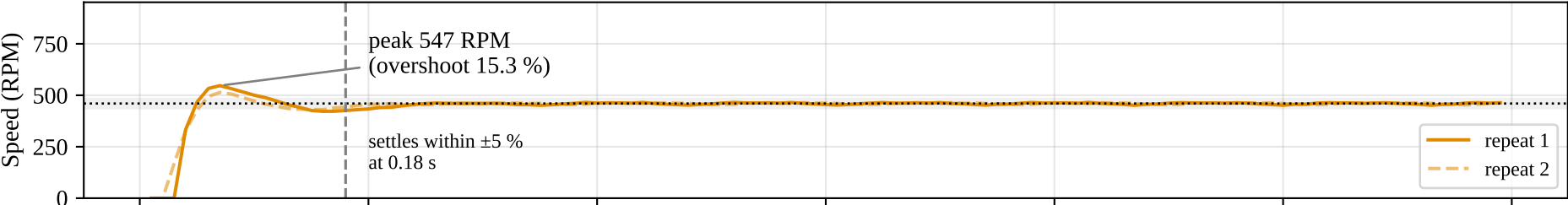
B1: α 0.5 → overshoot 15.3 %, settles in 0.18 s
