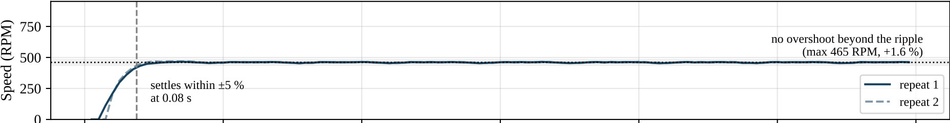
C3: Kp 0.8 → overshoot 1.6 %, settles in 0.08 s
