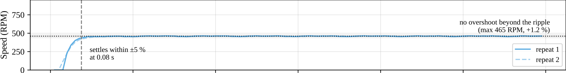
C2: Kp 1.0 → overshoot 1.2 %, settles in 0.08 s
