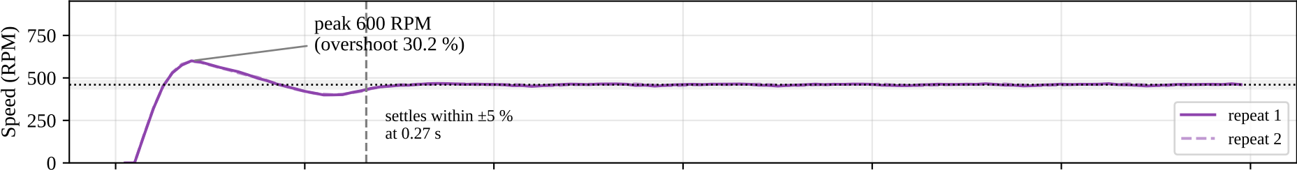
B2: α 0.3 → overshoot 30.2 %, settles in 0.27 s
