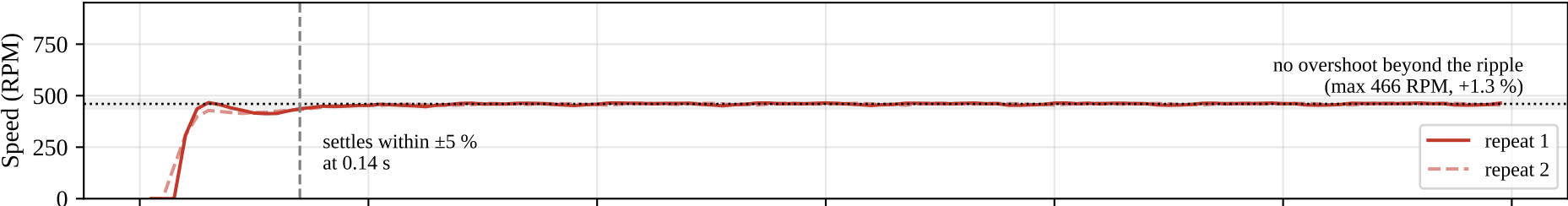
A: baseline (Kp 1.56, Ki 41.2) → overshoot 1.3 %, settles in 0.14 s
