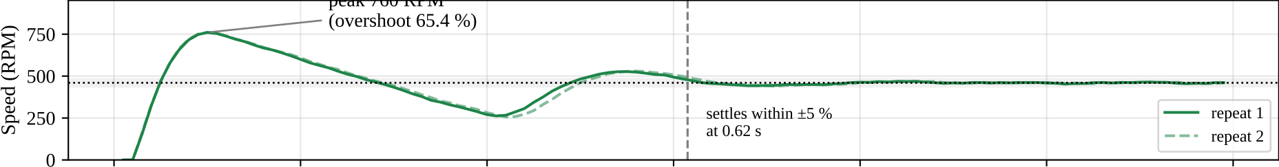
B3: α 0.15 → overshoot 65.4 %, settles in 0.62 s
