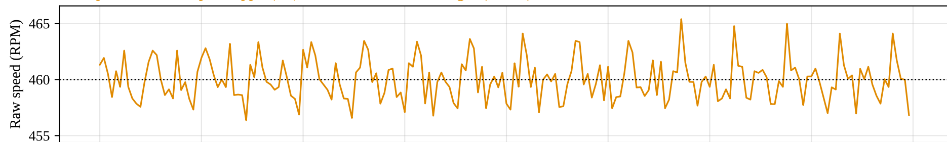
F1: Kp 0.8, \alpha 0.5 → speed ripple (std) 1.88 RPM = 0.41 % of target (-14 %)
