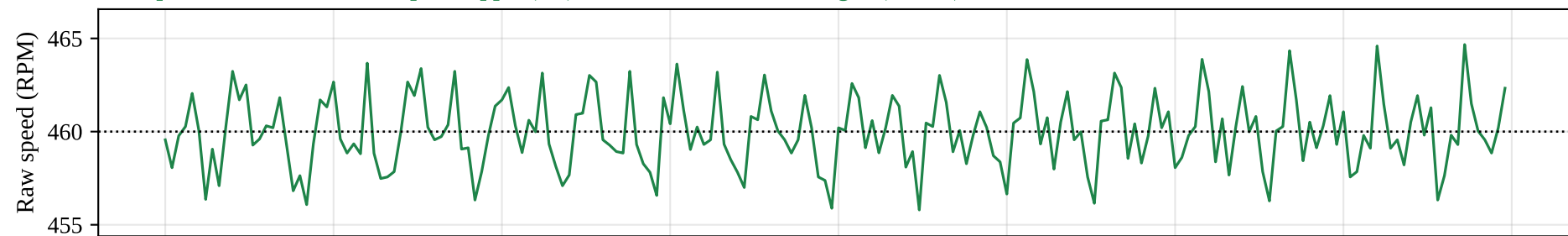
F3: Kp 0.8, Ki 25.0, \alpha 0.5 → speed ripple (std) 1.87 RPM = 0.41 % of target (-14 %)
