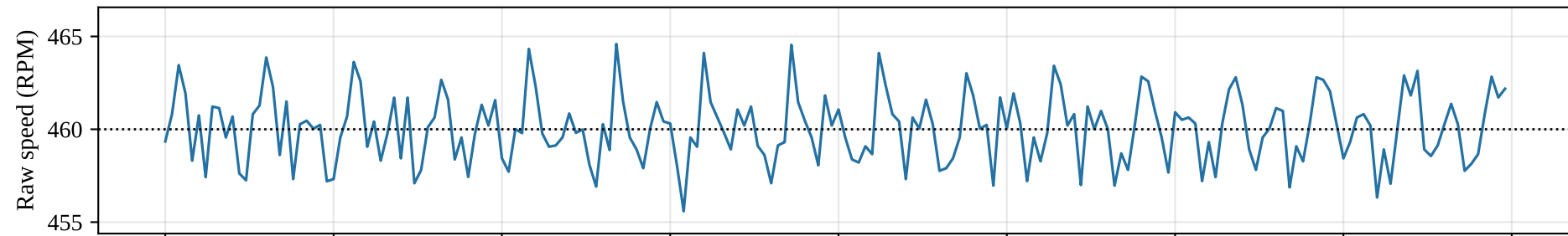
C3: Kp 0.8 → speed ripple (std) 1.93 RPM = 0.42 % of target (-11 %)
