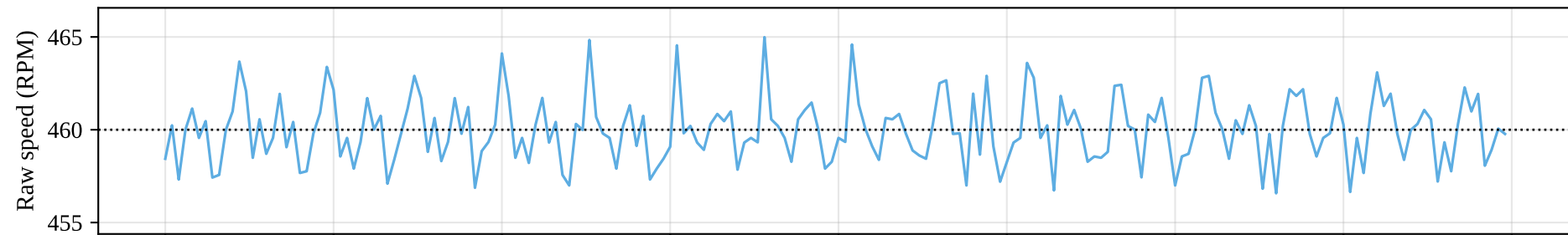
F4: Kp 0.8, Ki 15.0 → speed ripple (std) 1.90 RPM = 0.41 % of target (-12 %)
