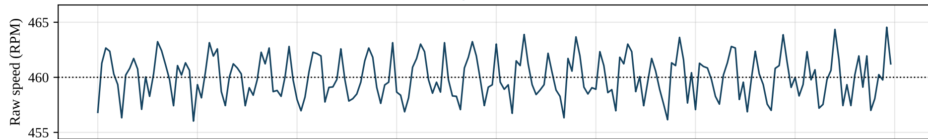
D3: Kp 1.0, \alpha 0.5 → speed ripple (std) 1.85 RPM = 0.40 % of target (-15 %)
