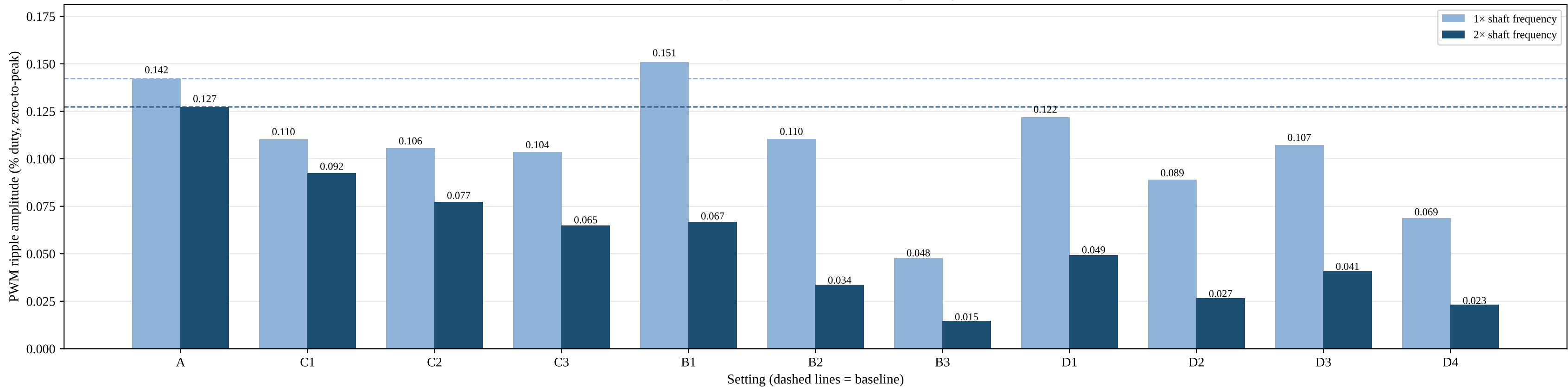
PWM ripple at the first two shaft orders, per setting
