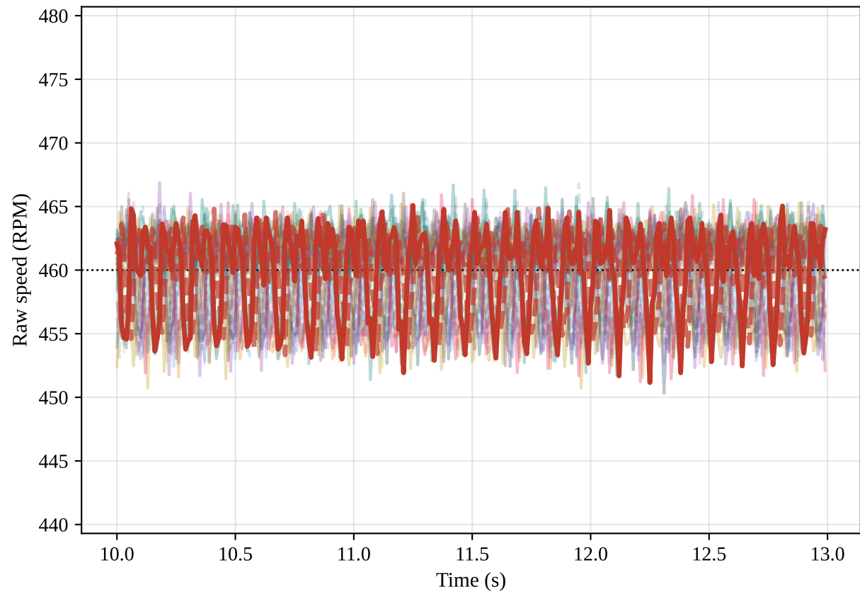
(b) Steady state (solid = run 1, dashed = run 2)
