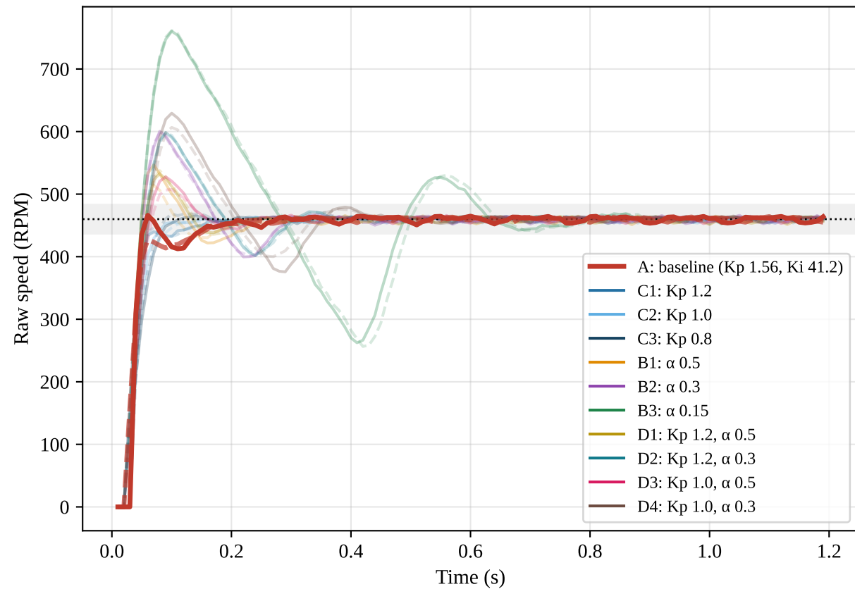
(a) Startup step 0 \rightarrow 460 RPM (grey band = \pm 5\% )
