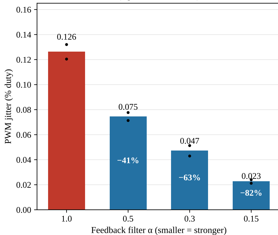
(b) Effect of filter \alpha ( K_p = 1.56 , K_i = 41.2 )
