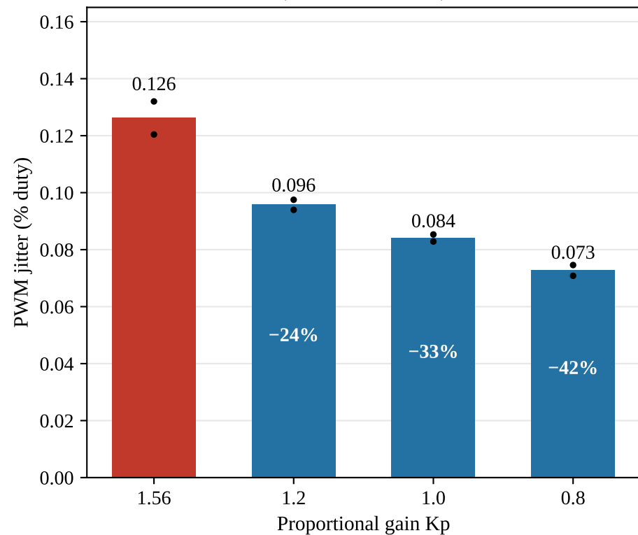
(a) Effect of K_p ( K_i = 41.2 , no filter)
