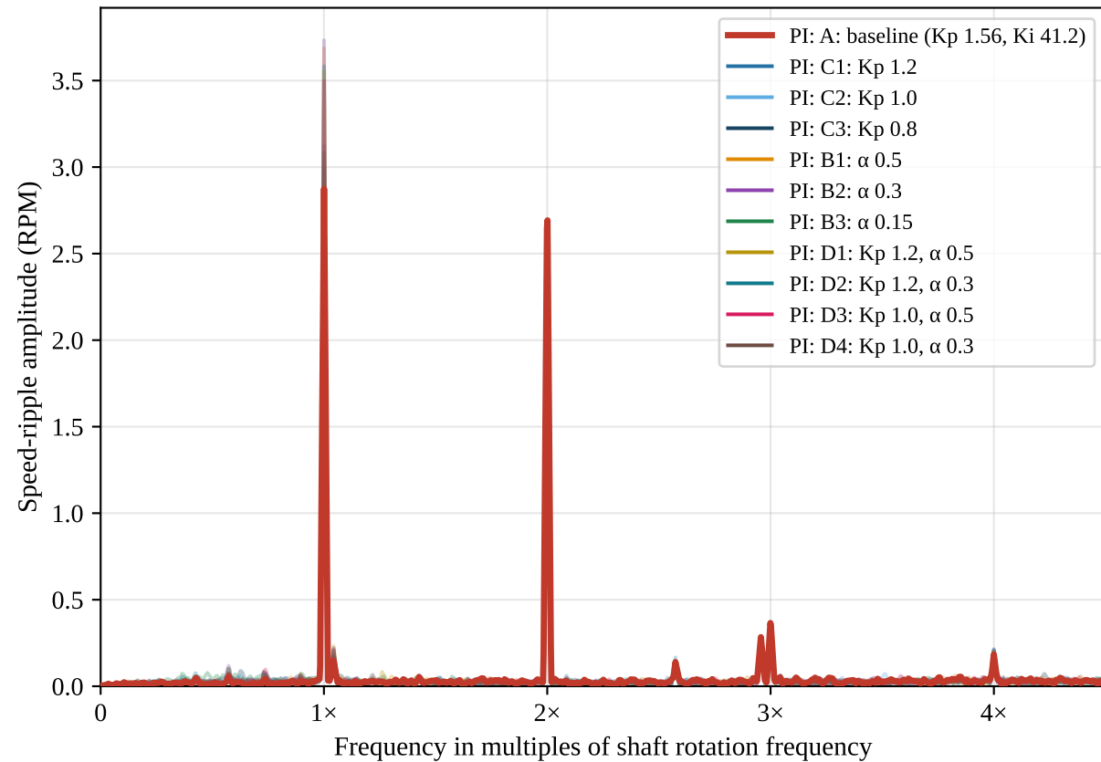
(a) Speed ripple
