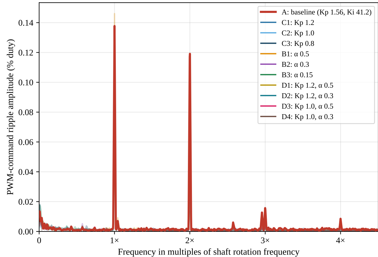
(b) PWM ripple reaching the motor
