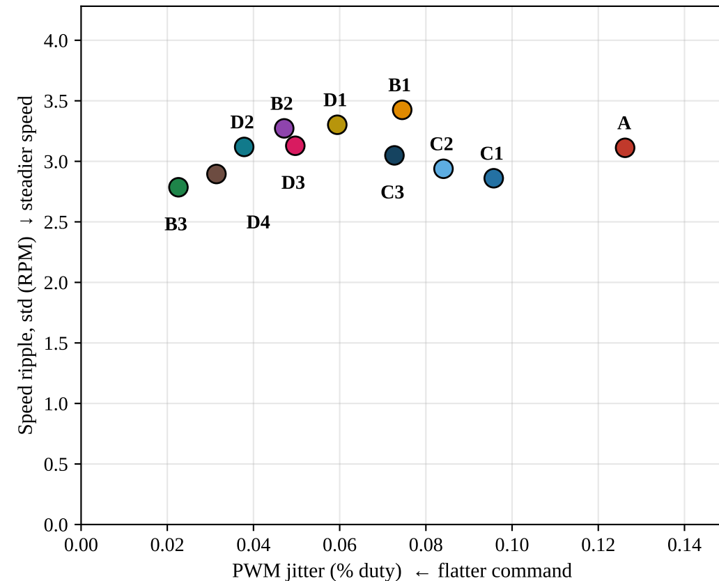
(c) Flatter PWM vs steadier speed
