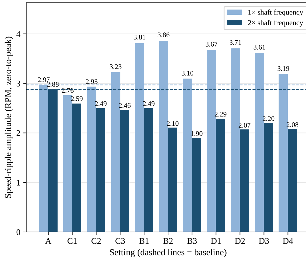
(b) Speed ripple at 1× and 2× shaft frequency
