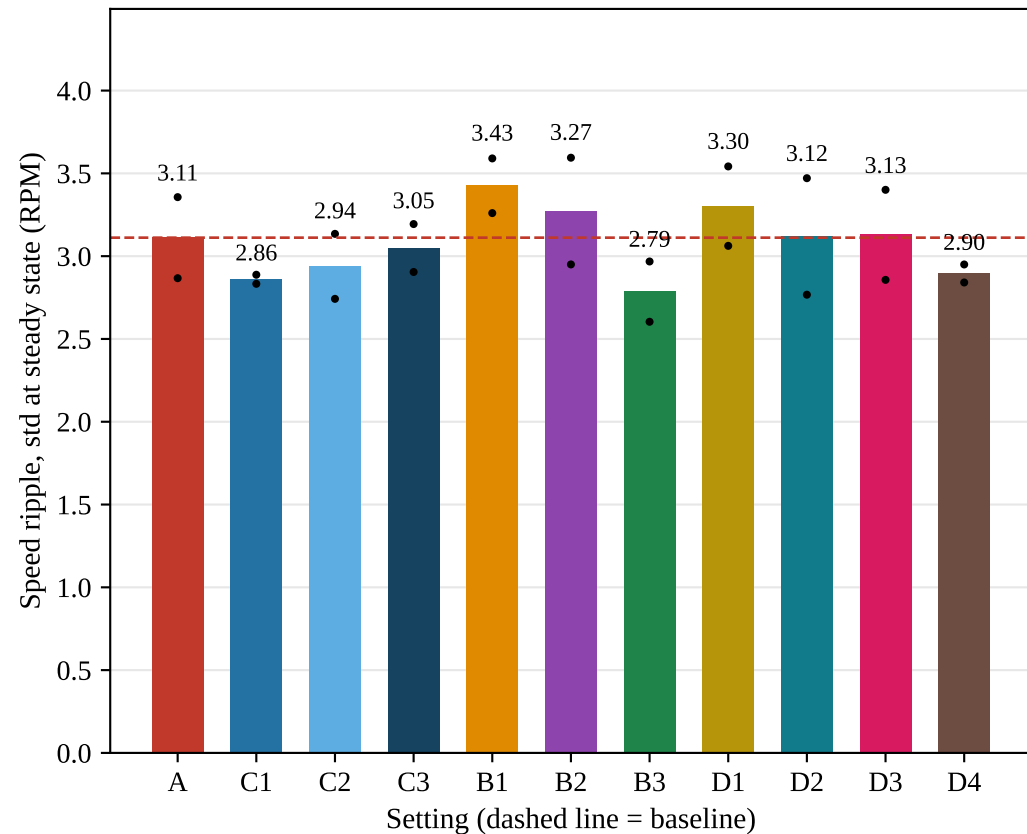
(a) Speed ripple per setting
