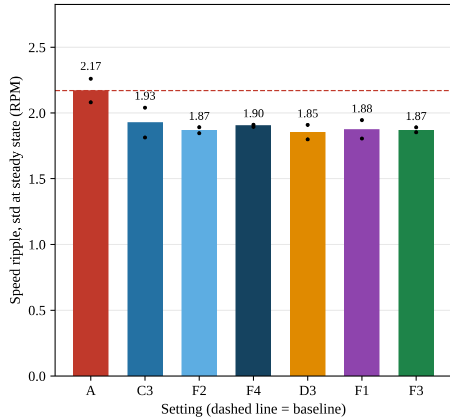
(a) Speed ripple per setting
