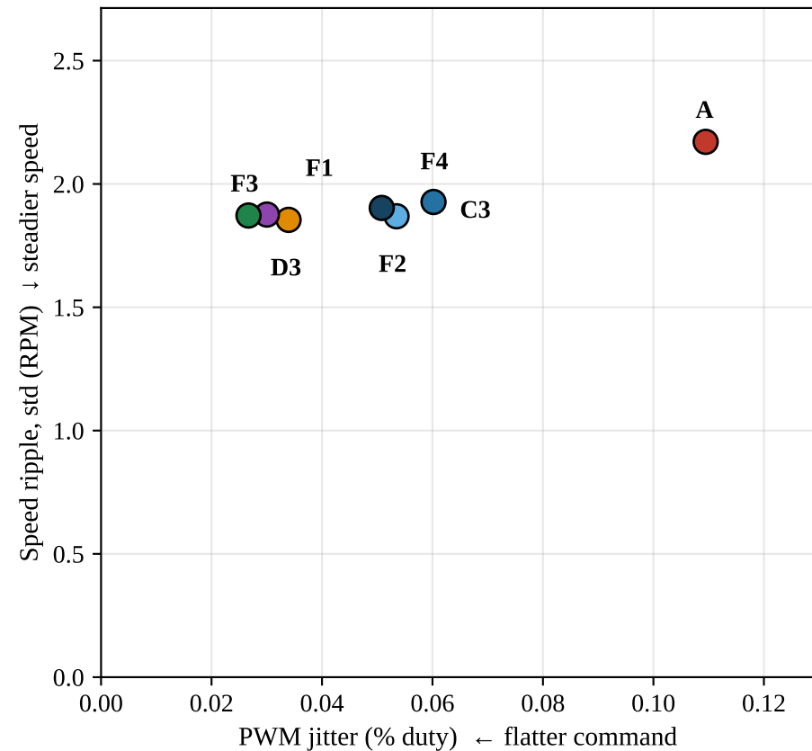
(c) Flatter PWM vs steadier speed
