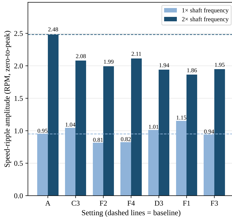
(b) Speed ripple at 1× and 2× shaft frequency
