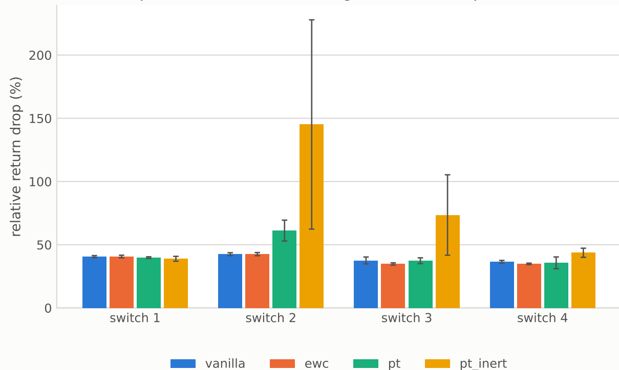
Return drop at each task switch (larger = worse adaptation)
