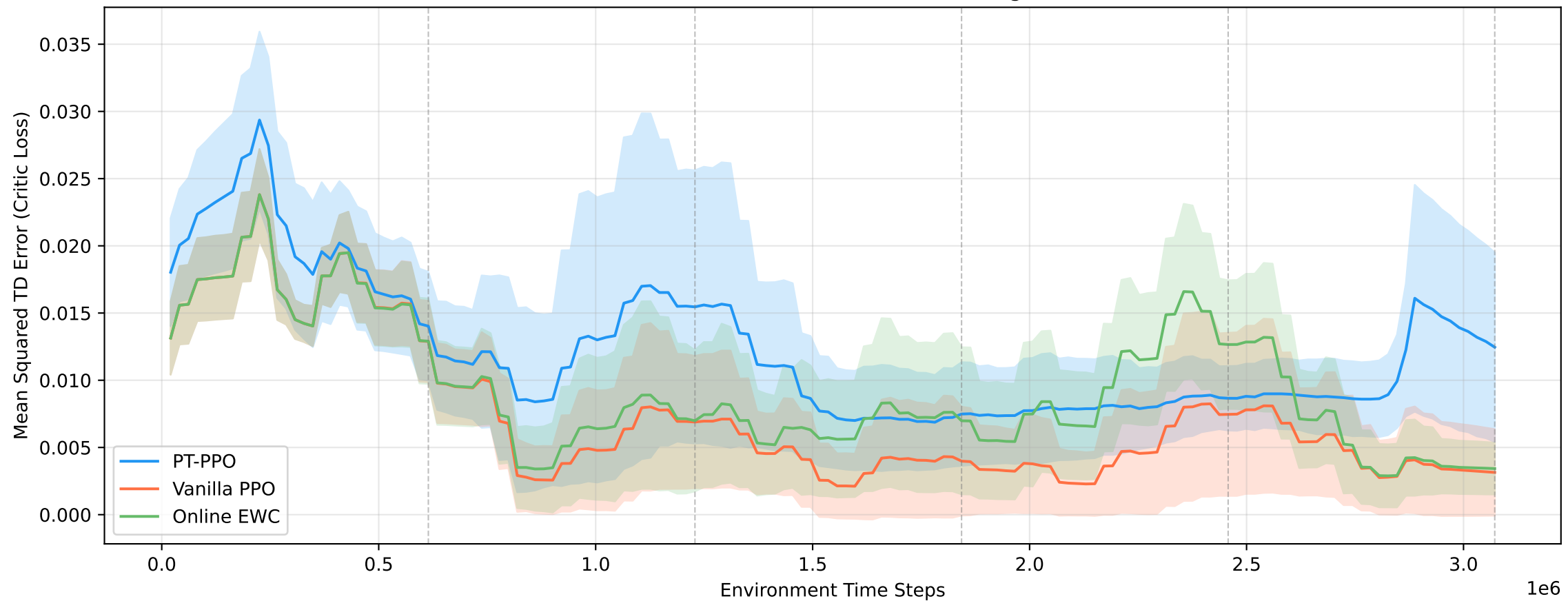
Continual HalfCheetah: Value Estimation TD Error Progression across Tasks
