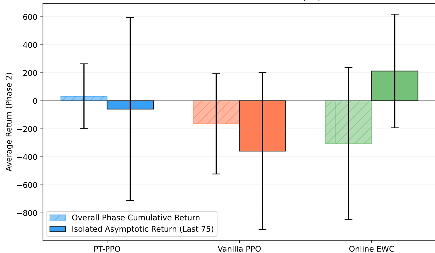
Phase 2: Overall Cumulative vs. Isolated Asymptotic Return
