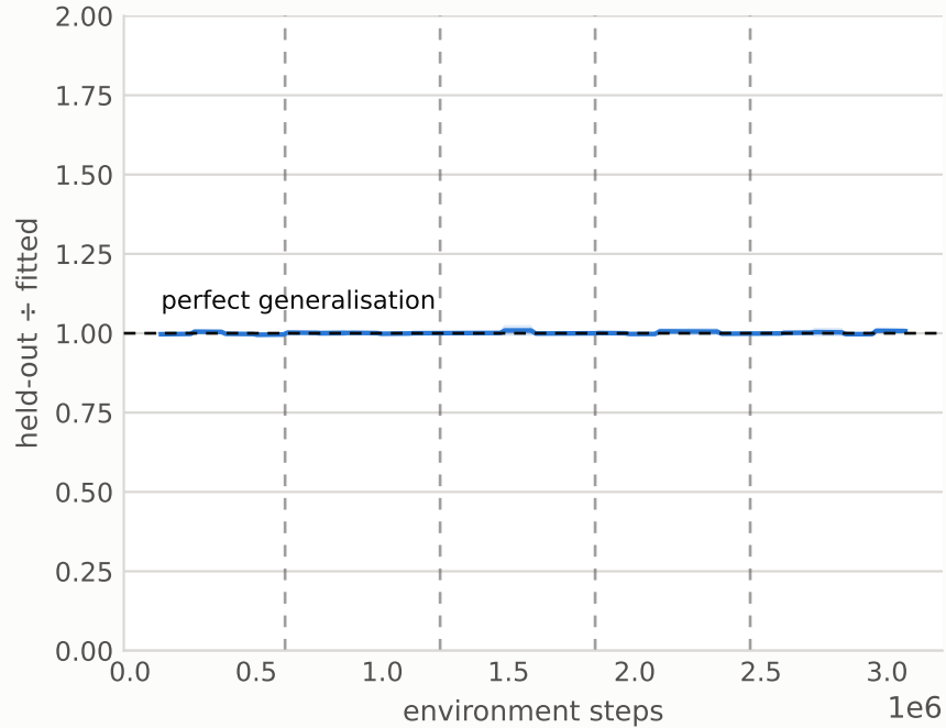
(b) ratio of the two — mean 1.001 memorisation would sit well below 1
