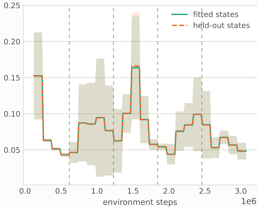
(a) how much of the transient the permanent takes up on states it fitted vs states it never saw
