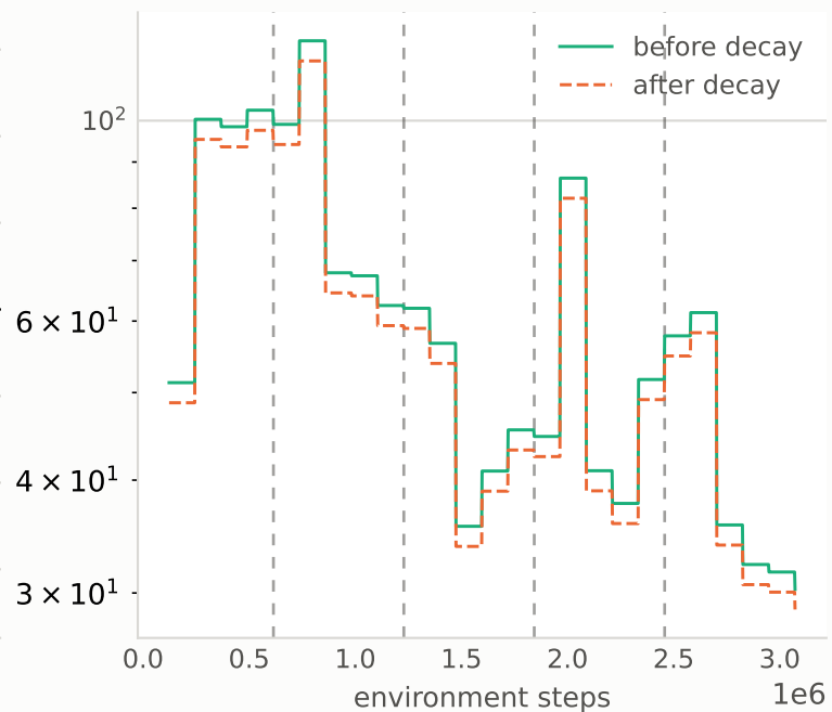
(c) L2 norm of the transient values over the batch
