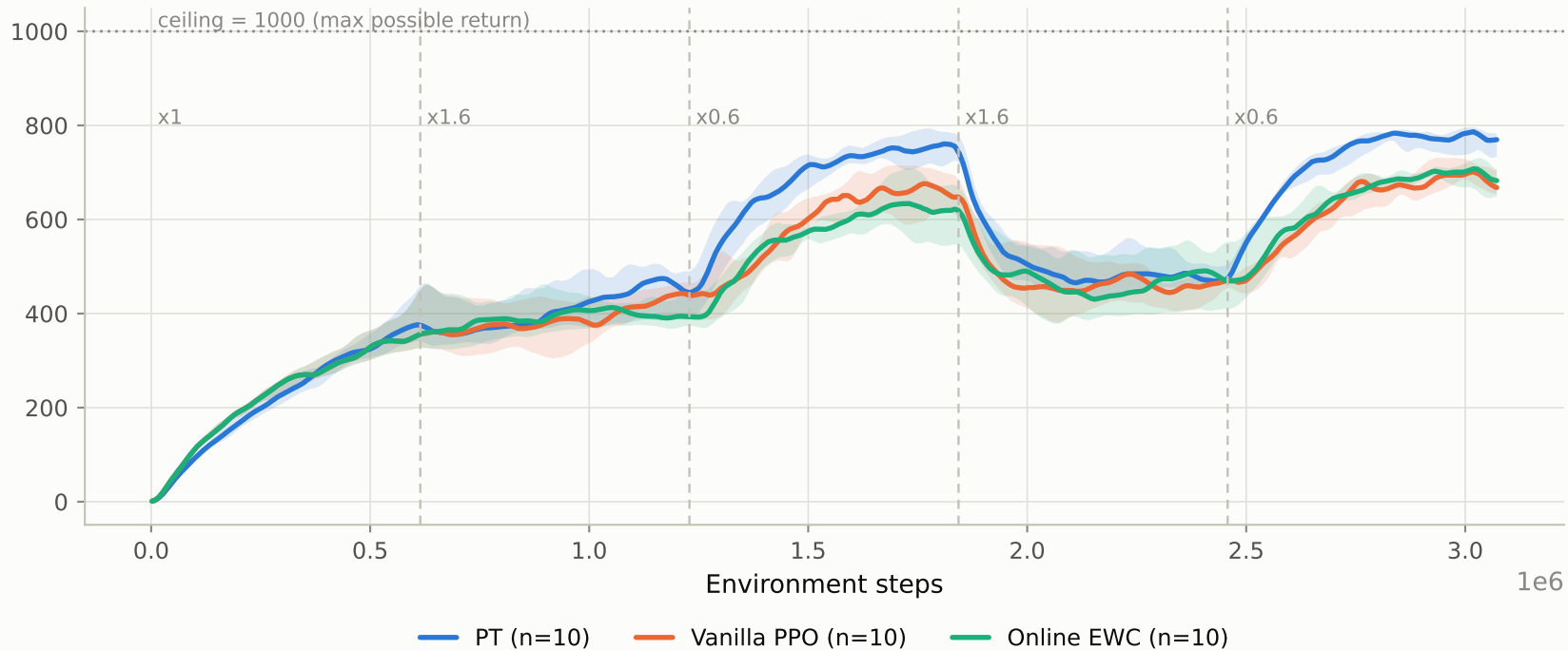
cartpole-swingup with changing pole: return through the task sequence
