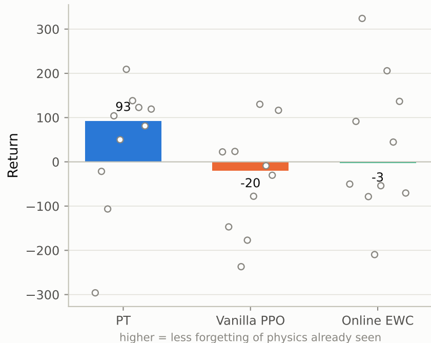
Backward transfer (BWT)
