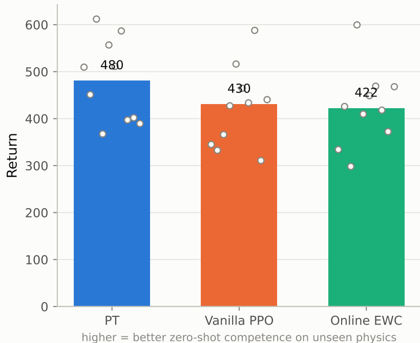
Forward transfer (FWT)
