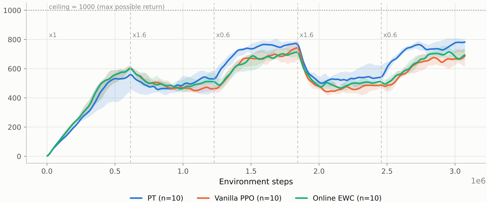
cartpole-swingup, standard PPO exploration: return through the task sequence
