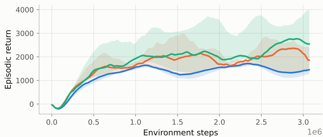
HalfCheetah - slow + fast drift (n=10)
