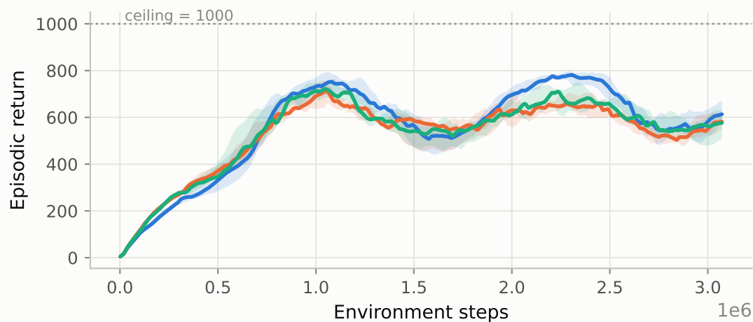
HalfCheetah - slow drift only (n=10)
