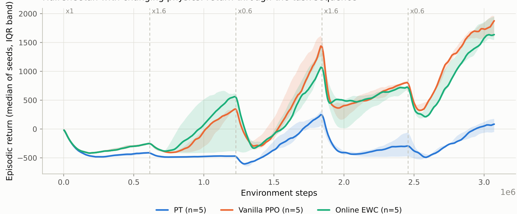
HalfCheetah with changing physics: return through the task sequence
