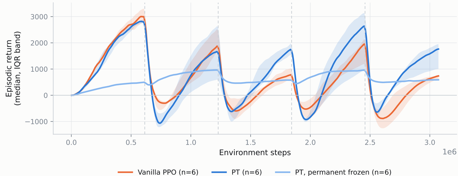
Reward flip, no boundary reset (Phase 1 archive)
