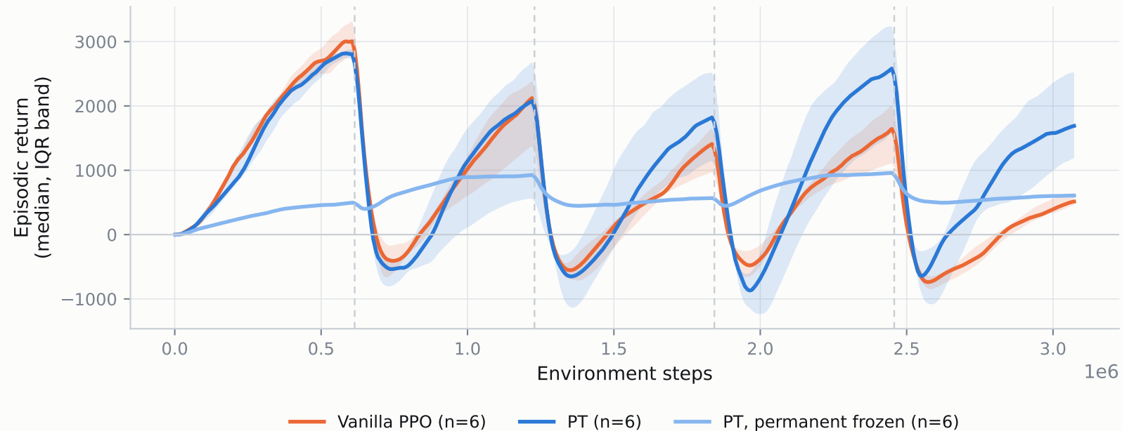
Reward flip, WITH boundary reset
