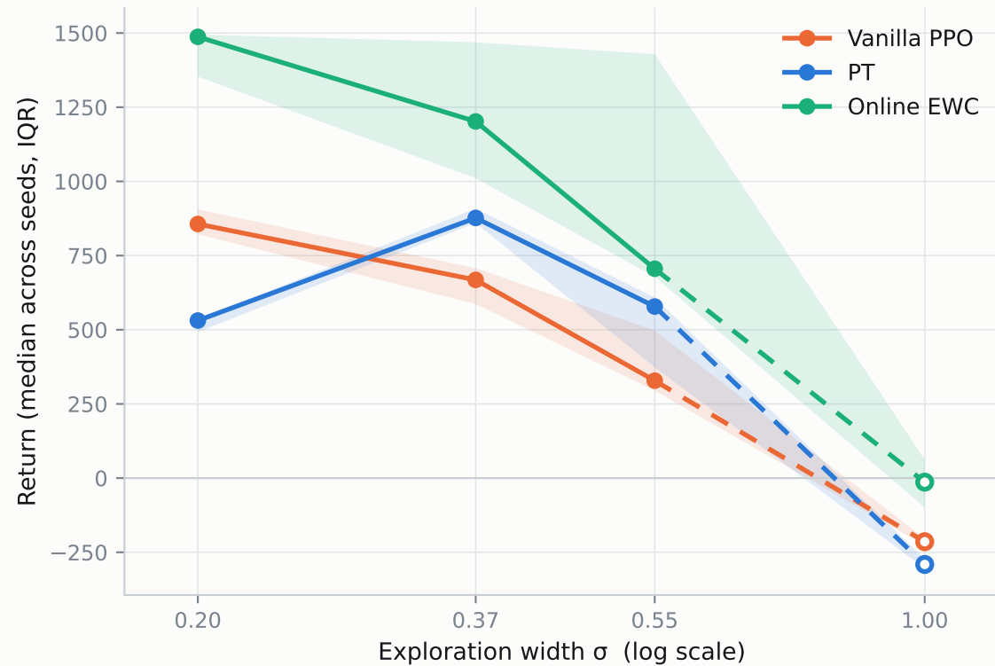
Every agent degrades with noise — but not in the same shape
