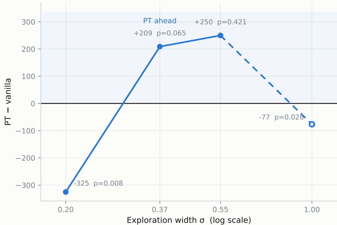
PT beats vanilla only in a band — and loses at both ends
